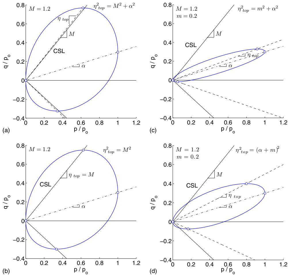
Fig. 2. Schematic illustration of four different choices for the factor N in the anisotropic elliptic yield surface: (a) Choice 1: N^2=M^2 ; (b) Choice 2: N^2=M^2-\alpha^2 ; (c) Choice 3: N^2=m^2 ; and (d) Choice 4: N^2=(\alpha+m)^2-\alpha^2 ; the stress-ratio quantity m is a measure of the difference between \eta_{top} and \alpha in (c) and (d)
