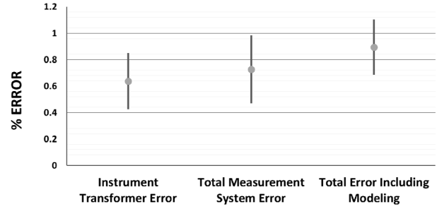
Figure 1. Error range for instrument transformers, total measurement system and modeling
