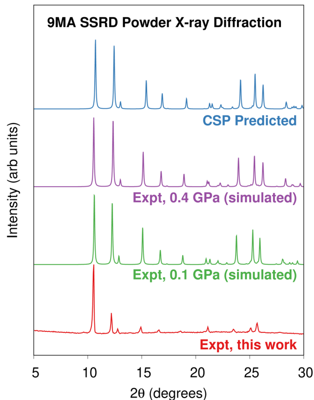
Fig. 4 Comparison of the powder X-ray diffractograms obtained on platelets of 9MA after 40 seconds illumination against the powder diffractograms simulated using the experimentally-reported 85 SSD crystal structures obtained at 0.1 and 0.4 GPa and the SSD structure generated via crystal structure prediction here.
