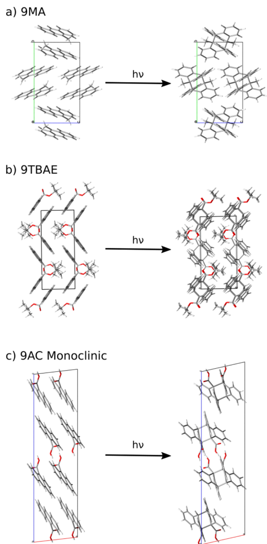
Fig. 3 The crystalline topochemical hypothesis generates the SSD based on the crystal packing of the monomer, as shown here for (a) 9MA , (b) 9TBAE , and (c) 9AC .
