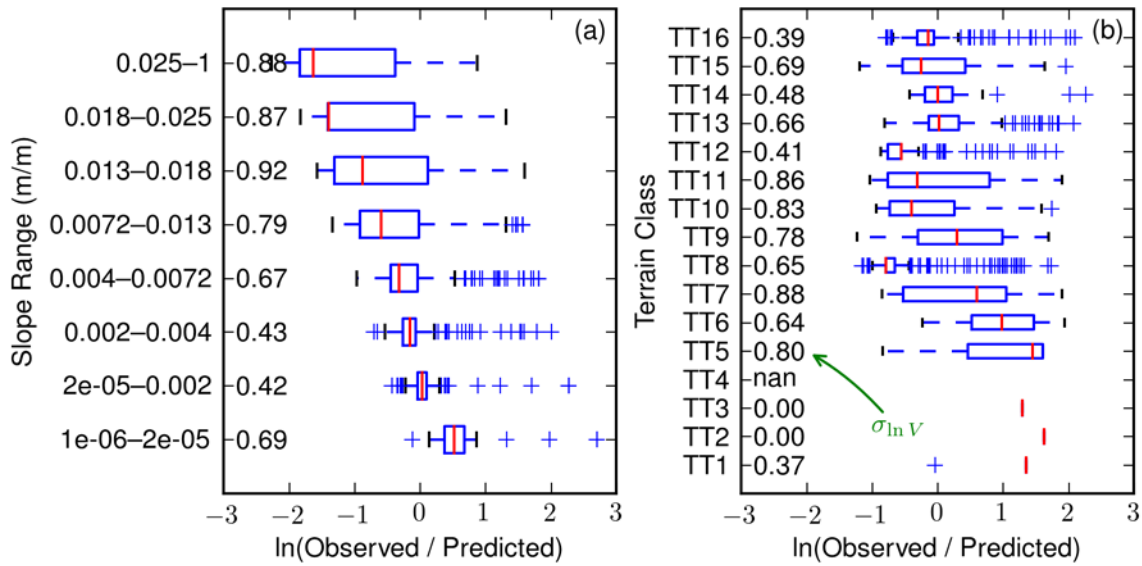
Figure 5. Boxplots of the residuals along with standard deviations ( \sigma_{\ln} ) for the slope- (a) and terrain- (b) based proxy methods. The total uncertainty ( \sigma_{\ln} ) of the slope- and terrain-based proxy methods is 0.92 and 0.72, respectively. Explanation of box plot format given with Figure 3.
