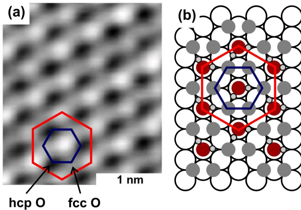
Figure 7. (Color online) (a) High resolution STM image from a water domain revealing the hexagonal structure of the adsorbed water. (b) Model structure of showing water adsorbed on the 2\text{O}(2\times 2)/\text{Ru}(0001) . Adapted from Ref. 1. STM image parameters: (a) 221 mV, 8 pA, (b) 221 mV, 7 pA.
