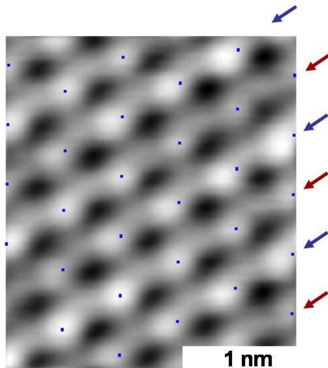
Figure 9. (Color online) Experimental STM image showing the presence of slight deviations from the perfect 2x2 alignment in the position of the maxima corresponding to water molecules, represented by the blue lattice. Every second row is slightly displaced.
