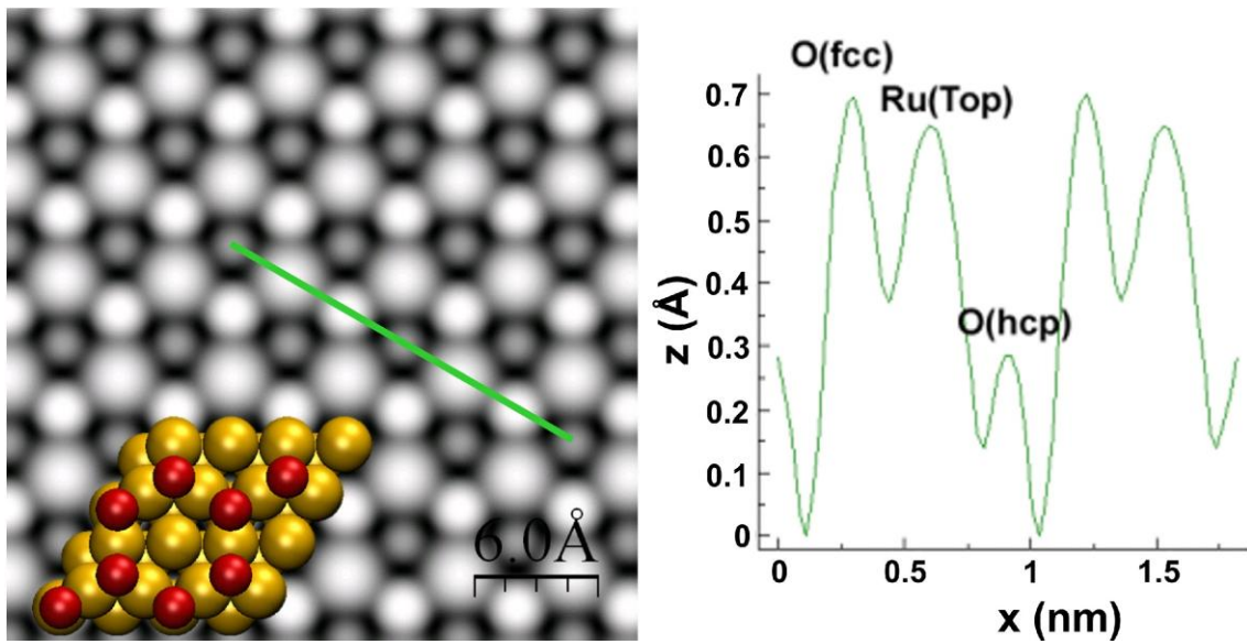
Figure 14. (Color online) Calculated constant current STM image at +400 meV bias, and topographic profile for the oxygen honeycomb reconstruction. Inset: red circles correspond to O atoms, yellow circles correspond Ru atoms.
