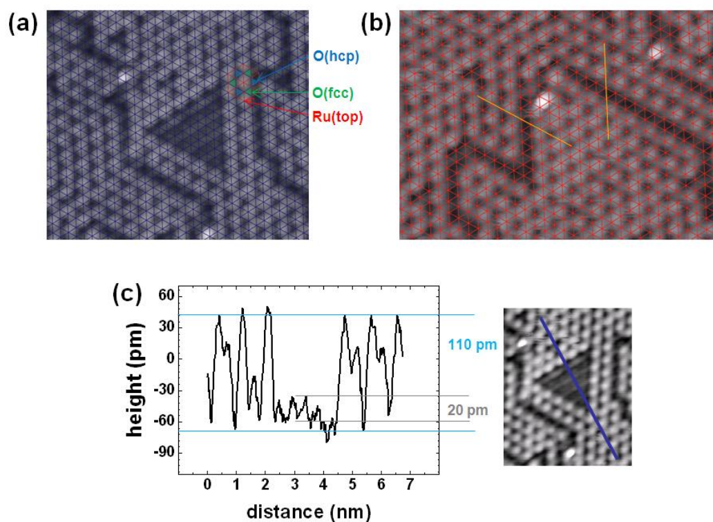
Figure 13. (Color online) (a) High resolution image (9.2nm x 6.8nm) of the O honeycomb structure with a small patch of the original O(2x1) structure. The resolution of the images in the O(2x1) patch is sufficient for identification of the adsorption sites in the surrounding honeycomb structure. The nodes of the superimposed lattice located over the white protrusions in the honeycomb structure represent Ru(0001) top sites. (b) The dark stripes are domain boundaries between different honeycomb patches as can be seen more clearly with the help of the yellow lines. The nodes of the lattice in (b) represent Ru(0001) fcc sites. (9nm x 5.2nm) (c) Section through the O(2x1) patch and honeycomb structure in the right image, showing that the corrugation in the honeycomb structure is about five times higher than in the O(2x1) structure. According to the simulated STM images, the double peak structure might be attributed to the O(fcc) and Ru top atoms. STM parameters: -21 mV and 11 pA.
