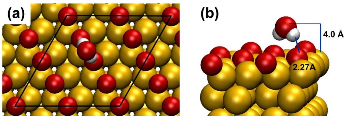
Figure 4. (Color online) Optimized model of a hypothetical water molecule adsorbed on an unmodified O(2x1)/Ru(0001): (a) top view and (b) side view. Two quite long and weak hydrogen bonds are formed with the oxygen atoms in the surface. The calculated binding energy of 86 meV is insufficient to ensure wetting.
