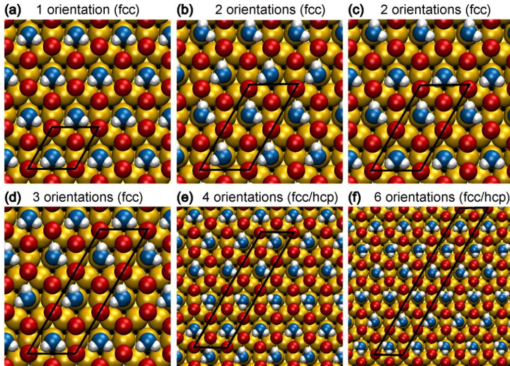
Figure 8. (Color online) Overview of relaxed geometries from the DFT calculations for different relative orientations of the water molecules within the layer. Figures (a)-(d) correspond to different configurations in which all the molecules are H-bonded to O(fcc) atoms. In panel (e) one molecule out of four is H-bonded to two O(hcp) atoms, and in panel (f) 50% of the molecules are H-bonded to O(hcp) atoms. In (a) all water dipoles are aligned, while in (b) their directions alternate. These two configurations are the most stable and are energetically degenerated, with an adsorption energy E_{\text{ads}} = 896 meV/H 2 O. The other configurations are slightly less stable with adsorption energies lower by 21 meV/H 2 O for (c), 17 meV/H 2 O for (d), 28 meV/H 2 O for (e), and 35 meV/H 2 O for (f).
