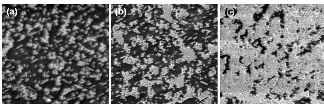
Figure 6. STM images of the \text{O}(2\times 1)/\text{Ru}(0001) surface with different amounts of water adsorbed at 140K: (a) 10-20% (b) 20-30% and (c) 75-85% water coverage. All images are 40 nm x 40 nm in size. STM image parameters: (a) -155 mV, 37 pA, (b) 221 mV, 8 pA, and (c) -385 mV, 4 pA.
