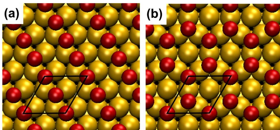
Figure 2. (Color online) Structures formed by oxygen on Ru(0001) at half monolayer coverage. Two possible surface geometries are shown, along with the 2x2-cell (dark lines) used in the DFT calculations. Yellow circles correspond to Ru atoms and red circles correspond to oxygen adsorbed on Ru hollow sites. (a) O(2x1) layer with all O atoms occupying hcp positions, and (b) 2O(2x2) honeycomb structure with half of the O atoms in hcp and half in fcc sites. Both systems were calculated and the O(2x1) structure found to be more stable by 231 meV per (2x2) cell.
