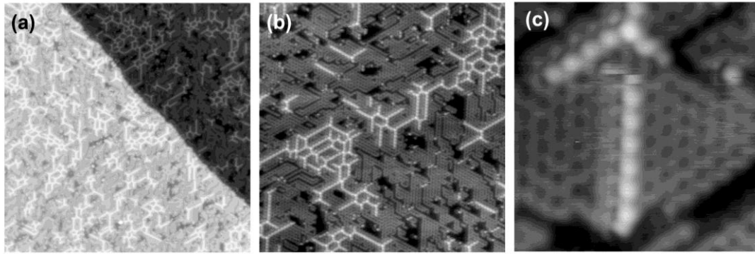
Figure 11. Water adsorbed at 140 K on the O/Ru(0001) surface followed by annealing to 180K. The residual water molecules form lines several nanometers long. The lines do not grow over monatomic steps nor decorate them as seen in (a). Image parameters: (a) 80 \text{ nm}^2 , -340 \text{ mV} , 9 \text{ pA} , (b) 40 \text{ nm}^2 , -310 \text{ mV} , 5.5 \text{ pA} , and (c) 6.6 \text{ nm}^2 , -309 \text{ mV} , 5.4 \text{ pA} .
