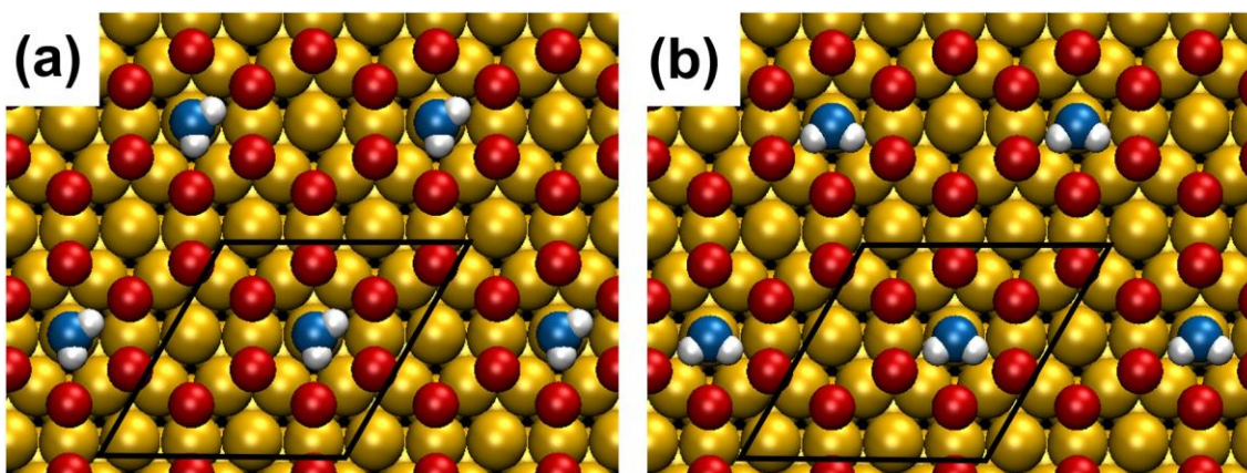
Figure 5. (Color online) Models of water adsorption structures on the 2\text{O}(2\times 2)/\text{Ru}(0001) honeycomb surface. A 4\times 4 cell (marked by the lines) was used for the calculations. The coverage of water is 0.25 ML. Yellow circles correspond to Ru atoms. Red circles correspond to oxygen atoms at hcp and fcc sites; the oxygen of the water molecule is represented in blue. The difference between the two structures is the orientation of the water molecule: (a) H atoms point towards the O(hcp) atoms; (b) H atoms point towards the O(fcc) atoms. Adsorption energies are given in the last row of Table I. The O(fcc)-oriented molecules are \sim 60 meV more stable.
