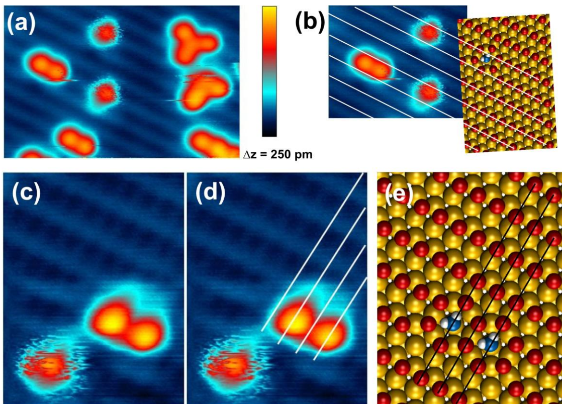
Figure 3. (Color online) (a) STM image showing individual water molecules, and groups of two and three molecules in adjacent sites on a O(2x1)/Ru(0001) adsorbed at 140K. During imaging at 7K, clusters of neighboring molecules are stable, while isolated molecules are vibrating. (5.8 nm x 3.8 nm, -380 mV and 5.4 pA). The schematic in (b) shows that water molecules adsorb between the oxygen rows. The Ru atoms are represented in yellow, surface oxygen in red and the oxygen of the water molecule in blue. (c)-(d) Images showing isolated water molecules and pairs of molecules on a well resolved image of the O(2x1)/Ru(0001) surface (2.9 nm x 4.7 nm, -245 mV, and 10 pA). The schematic drawing in (e) shows the location of the water molecules relative to the 2x1 oxygen lattice.
