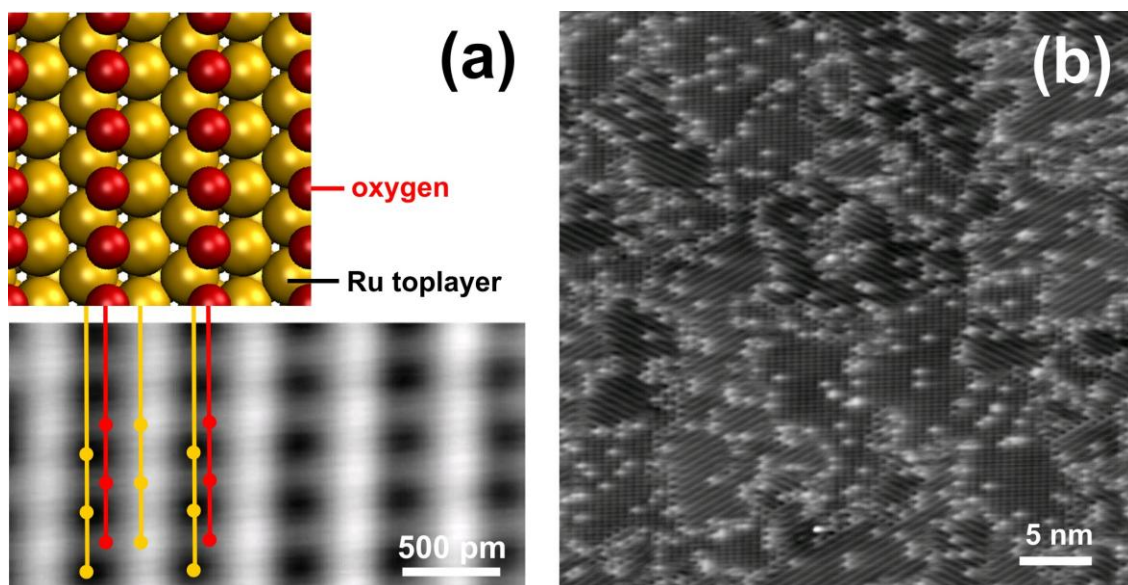
Figure 1. (Color online) (a) Atoms resolved STM image (bottom) and schematic representation (top) of the O(2x1)/Ru(0001) surface. Red circles represent the oxygen atoms, yellow represent the Ru atoms. (b) Large scan area image of the O(2x1)/Ru(0001) surface, showing different domains rotated 120^\circ with respect to each other. White spots correspond to O vacancies. Imaging parameters: (a)-(b) 21.5 mV, 89.6 pA.
