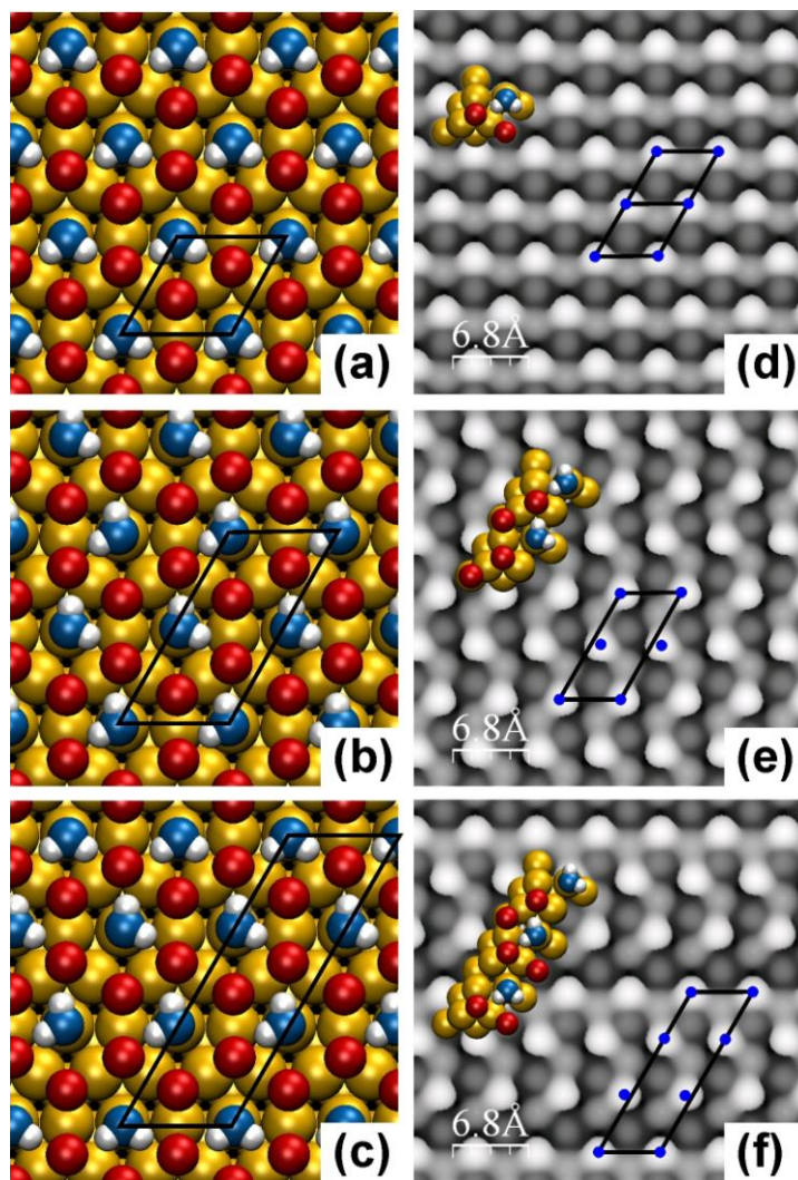
Figure 10. (Color online) (a)-(c) Optimal configurations for the adsorption of water molecules on the oxygen-honeycomb reconstruction showing (a) one, (b) two, and (c) three different molecular orientations. Structures (a) and (b) are energetically degenerate, while (c) is slightly less optimal by \sim 17 meV/H 2 O. In all the configurations, the water molecules are slightly displaced ( \sim 0.2 Å) along the xy-plane, with respect to the Ru top sites, in order to form hydrogen bonds with the O(fcc) atoms (bond length 2.25 Å). (d)-(f) Corresponding simulated constant current images at +400 meV bias. In panels (e) and (f) the slightly displaced centers of the molecular protrusion are marked in blue.
