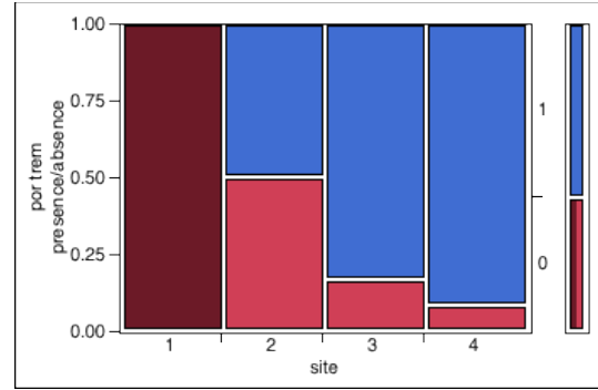
Fig. 8 Presence or absence of Porites Trematodiasis by site. The 1 represents the presence and the 0 the absence.
