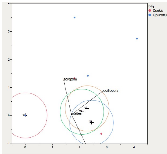
Fig. 7 Coral species composition canonical by site and bay. Each colored circle is a separate site combining both bays and both east and west sides of the bays, but the same relative distance from the river mouth. The coral four coral species are the determining factors for how they grouped. The red and blue dots represent the respective bays.
