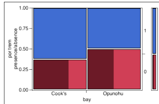
Fig. 9 Presence/absence of porites trematodiasis in Cook's and Opunohu Bays. The 1 represents the presence and the 0 represents the absence.
