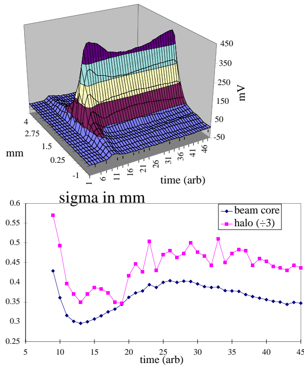
Figure 3: Beam profile data at focus
