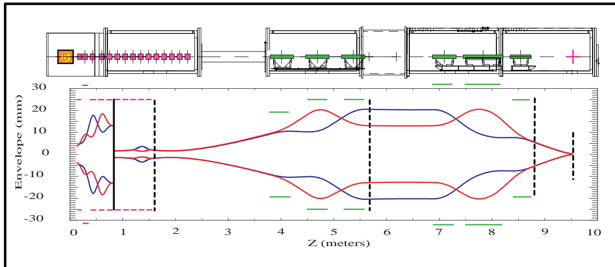
Figure 1: Experimental layout and beam envelopes.
