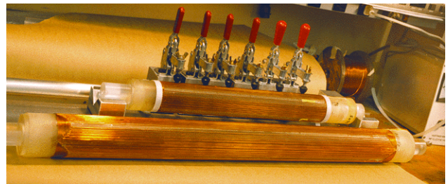
Figure 2: Magnetic quadrupoles and winding rig
