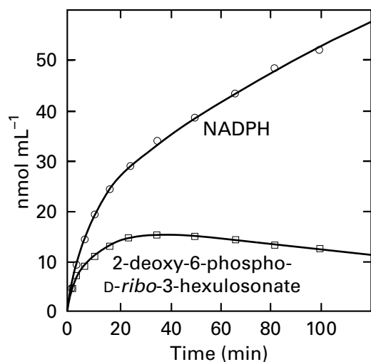
Figure 5-6: Kinetics of formation of 2-deoxy-6-phospho-D-ribo-3-hexulosonate and NADPH in the unnatural reaction catalyzed by phosphogluconate dehydrogenase (NADP + -dependent, decarboxylating). 273 To the reaction mixture at 20 °C (final volume of 1 mL buffered at pH 8.0) were added 1.0 μmol of 2-deoxy-6-phospho-D-gluconate, 1.2 μmol of NADP + , and 0.68 unit of phosphogluconate dehydrogenase. (○) The increases in the concentration of NADPH (nanomoles milliliter -1 ) were followed as a function of the respective intervals (minutes) by the absorbance of the solution at 340 nm. (□) The concentrations of 2-deoxy-6-phospho-D-ribo-3-hexulosonate (nanomoles milliliter -1 ) were assessed at intervals (minutes) by withdrawing samples and forming a formazan derivative from the β-oxo carboxylic acid by reaction with diazotized 4-nitroaniline.
