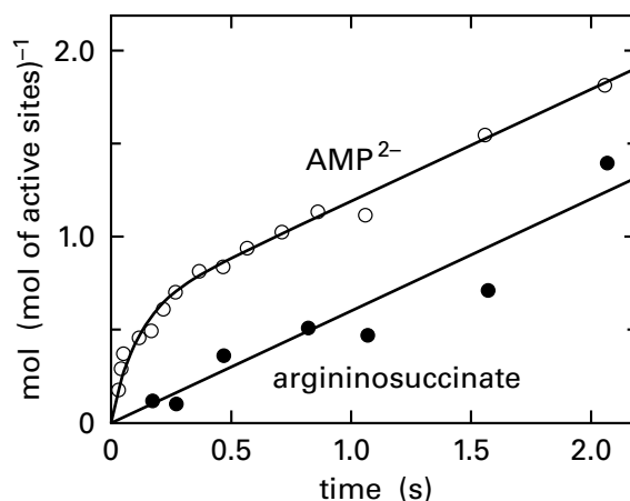
Figure 5-32: Burst in formation of \text{AMP}^{2-} observed by quenched flow during the reaction of argininosuccinate synthase. 948 A solution of bovine argininosuccinate synthase ( 34 \mu\text{M} in active sites) was mixed with an equal volume of a solution containing 5.0 \text{ mM} L-citrulline, 2.0 \text{ mM} \text{MgATP}^{2-} , and 5.0 \text{ mM} L-aspartate. Both solutions contained 9 \text{ mM} \text{MgCl}_2 and 100 \text{ mM} 2-amino-2-(hydroxymethyl)propane-1,3-diol chloride, \text{pH } 8.0 and 22^\circ\text{C} . The two solutions were mixed in a mixing chamber, the mixture flowed through a tube of a particular length, and the mixture was then quenched with 0.25 \text{ M} \text{H}_2\text{SO}_4 . This procedure was repeated with the same two solutions, varying the time each mixture spent between the mixing chamber and the quench solution by choosing different lengths of tubing. A portion of each quenched solution was submitted to high-pressure liquid chromatography to isolate \text{AMP}^{2-} , which was quantified by its absorbance. Another portion of each quenched solution was brought to \text{pH } 7 and mixed with a solution of bovine argininosuccinate lyase to hydrolyze 2-( N^{\omega} -L-arginino)succinate (argininosuccinate) to fumarate and L-arginine. Each sample was then submitted to high-pressure liquid chromatography to isolate fumarate, which was quantified by its absorbance. The moles of \text{AMP}^{2-} (mole of active sites of argininosuccinate synthase) ^{-1} and the moles of 2-( N^{\omega} -L-arginino)succinate (mole of active sites of argininosuccinate synthase) ^{-1} in the reaction mixtures are plotted as a function of the intervals between mixing and quenching (seconds).
