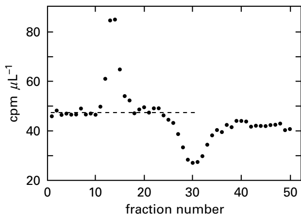
Figure 3-19: Determination of the concentration of histidinol bound to histidinol dehydrogenase by molecular exclusion. 161 A column (0.5 cm × 7.5 cm) of beaded, crosslinked dextran (Sephadex G-50) was equilibrated with buffer containing 0.5 mM MnCl 2 , 1 mM potassium phosphate, 1.0 \times 10^5 counts per minute mL -1 [ 32 P]phosphate, 10 μM [ 3 H]histidinol ( 4.7 \times 10^6 counts per minute μmol -1 ) and 50 mM sodium glycinate at pH 9.05. A sample of histidinol dehydrogenase dissolved in 100 μL of the buffer used to equilibrate the column was applied, and the column was eluted with 2.8 mL of the buffer. Each fraction from the column was one drop of effluent (48–53 μL). To determine the counts per minute (cpm) of [ 3 H]histidinol for every microliter of solution in each fraction, the exact volume of each drop was determined from the counts per minute of [ 32 P]phosphate, and the counts per minute of [ 3 H]histidinol in each fraction was divided by that volume. The counts per minute of [ 3 H]histidinol in each microliter of effluent (cpm μL -1 ) is presented as a function of the fraction number. The free concentration of histidinol is represented by the counts per minute microliter -1 in the effluent before and after the excluded volume of the column (fractions 11–17), as indicated by the dashed line. The counts per minute in excess of those representing the free concentration of [ 3 H]histidinol in each fraction were summed over the excluded volume and converted to nanomoles of bound histidinol.
