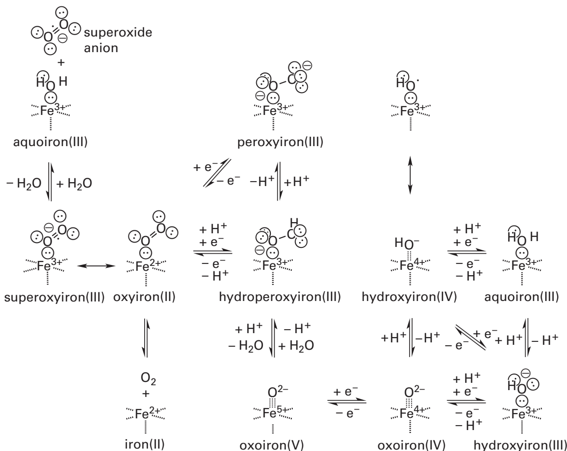
Figure 2–50: Complexes formed between iron ions and the different oxidation states of oxygen. Superoxide radical anion combines with Fe^{3+} (top) or molecular oxygen combines with Fe^{2+} (bottom) to produce the same complex, oxyiron(II), which stereochemically resembles a superoxide radical anion on Fe^{3+} but has the oxygen–oxygen bond length of molecular oxygen. The addition of a hydron and an electron to this complex produces hydroperoxyiron(III), identical to the complex resulting from the addition of hydroperoxide ion, the conjugate base of hydrogen peroxide, to Fe^{3+} . Hydroperoxyiron(III) is the conjugate acid of peroxyiron(III). The addition of a hydron to the distal oxygen in hydroperoxyiron(III) and the heterolytic loss of
