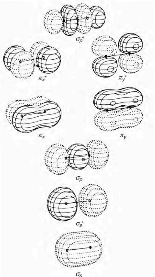
Figure 2–45: One of several ways to depict the molecular orbitals of the O_2 molecule. 675 The drawings of the individual molecular orbitals are distributed and labeled as they are in 2–87. The two lowest, cylindrically symmetric \sigma molecular orbitals along the line of centers between the two oxygen atoms ( \sigma_s and \sigma_s^* ) are formed from the overlap of two s atomic orbitals, one from each oxygen atom. The two highest cylindrically symmetric \sigma molecular orbitals along the line of centers between the two oxygen atoms ( \sigma_p and \sigma_p^* ) are formed from the overlap of two p_z atomic orbitals, one from each oxygen atom. The two pairs of \pi molecular orbitals, which are orthogonal and degenerate to each other, are formed from the p_x orbitals ( \pi_x and \pi_x^* ) and the p_y orbitals ( \pi_y and \pi_y^* ) of the two oxygen atoms. In the ground state, the distribution of electrons in these orbitals is as in 2–87. Reprinted with permission from reference 675. Copyright 1979 Annual Reviews, Inc.
