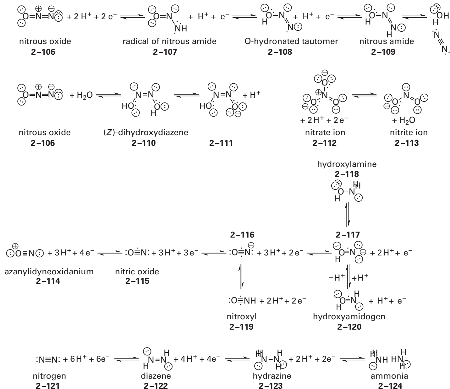
Figure 2-56: Oxides and hydrides of nitrogen and their inter-conversion by oxidation-reduction. Dihydroxydiazene and nitroxyl exist in the gas phase in equilibrium with each other, and dihydroxydiazene decomposes in water. 1673 Hydroxyamid-
