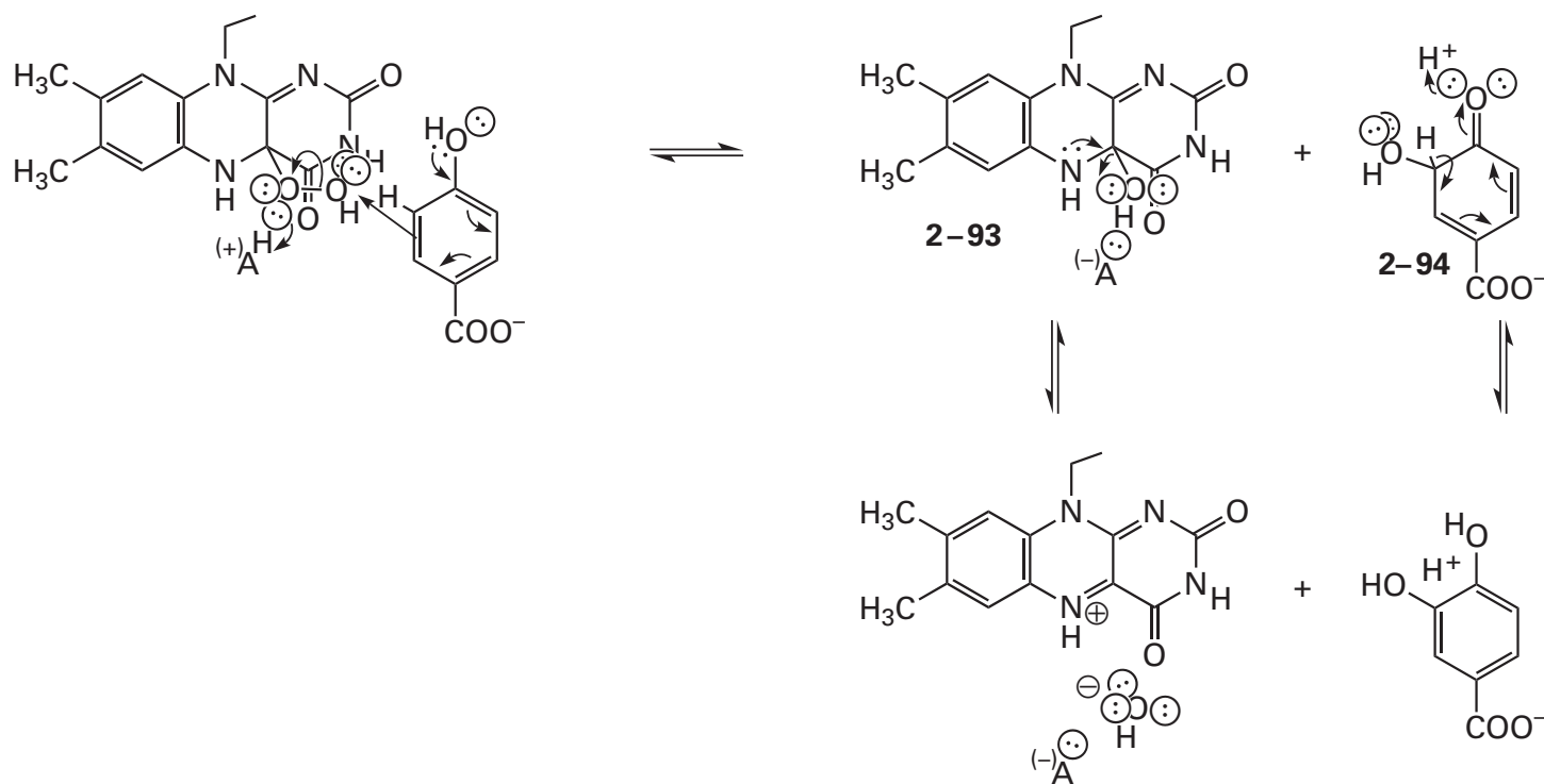
Figure 2-48: Mechanism for the hydroxylation of 4-hydroxybenzoate by 4a-hydroperoxyflavin in the reaction catalyzed by the flavoenzyme 4-hydroxybenzoate 3-monooxygenase (Equation 2-212). The electrophilic hydroperoxy group of the 4a-hydroperoxyflavin, formed by the reaction of molecular oxygen with reduced flavin, is attacked by a pair of the nucleophilic \pi electrons in the aromatic \pi molecular orbital system of the 4-hydroxyphenyl group of the 4-hydroxybenzoate at the same time that a
