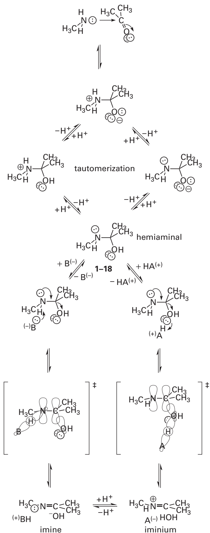
Figure 1-7: Addition of an amine to a carbonyl compound. The conjugate base of the amine adds to the carbonyl group to produce the zwitterion. A base in the solvent removes a hydron from the ammonium ion and an acid in the solvent adds a hydron to the oxyanion to produce the hemiaminal (1-18). The hemiaminal is susceptible to elimination in a reaction catalyzed by a general base 87 or a general acid. 86,88 In the reaction catalyzed by a general base, a hydron is removed from the nitrogen at the same time that an orthogonal lone pair of electrons on the same nitrogen pushes out the leaving group, a hydroxide ion. In the reaction catalyzed by a general acid, a hydron is added to a lone pair of electrons on the dissociating oxygen at the same time that the lone pair of electrons on nitrogen is pushing out the orthogonal \sigma bond to the same oxygen. In both the transition state for the reaction catalyzed by the general base and the transition state for the reaction catalyzed by the general acid, six atomic orbitals mix to form the respective transition states.
