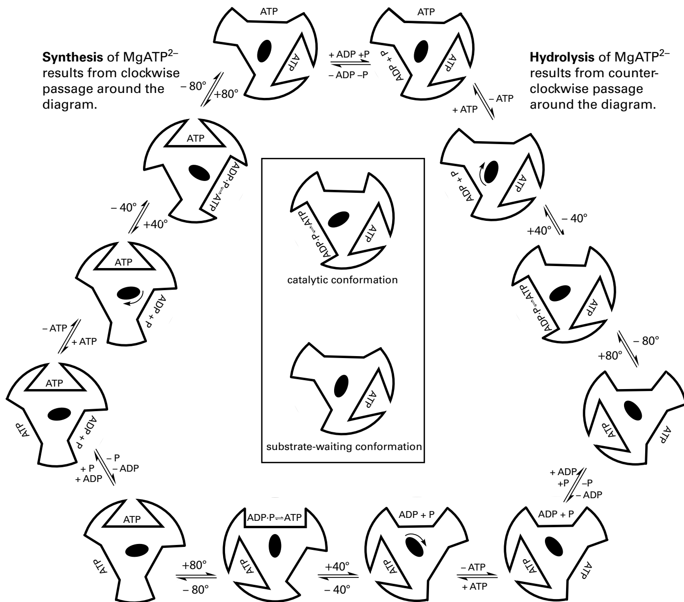
Figure 6-50: Revision of the diagram of Figure 6-45 to incorporate the properties of the intermediate conformation that, during hydrolysis of MgATP 2- , follows a discontinuous rotation of -80^\circ and precedes a discontinuous rotation of -40^\circ to complete a step of -120^\circ (Figure 6-49). The diagrammatic representations for each of the three conformations of the \alpha\beta heterodimer in the two different global conformations are defined within the box in the center. In this diagram, the two intermediate rotations comprise the sides of the equilateral triangle with the catalytic
