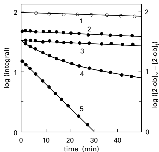
Figure 5-16: Isotopic exchange of hydrogens on the \alpha and \beta carbons of L-methionine, as well as loss of methanethiol during the overall reaction, for the enzymatic reaction catalyzed by methionine \gamma -lyase from P. putida . 821 A solution (0.5 mL) was prepared at p 2 H 8.6 and 28 °C that contained 100 mM L-methionine in ^2\text{H}_2\text{O} (99.8% isotopic enrichment). The reaction was initiated by adding 0.8 nmol of active sites of methionine \gamma -lyase, and the solution was placed in a nuclear magnetic resonance spectrometer. At various intervals, spectra were recorded. Amplitudes of the absorptions in spectra from the \alpha -hydrogen (curve 5), the \beta -hydrogens (curve 4), the \gamma -hydrogens (curve 3), and the S-methyl hydrogens (curve 2) were determined by integration of the respective peaks on each spectrum. The common logarithms of these integrals are plotted (●) as a function of the intervals (minutes) that had elapsed from initiation of the reaction to the time at which each peak was recorded. The two \beta -hydrogens exchange at different rates, and this heterogeneity accounts for the nonlinear behavior of their absorption. At various intervals, samples were withdrawn and quenched, and the appearance of 2-oxobutanoate was followed by reacting the ketone with 3-methyl-2-benzothiozalone. The disappearance of L-methionine as a result of the enzymatic reaction was assumed to be equal to the difference between the concentration (millimolar) of 2-oxobutanoate (2-ob) at infinite time ( [2\text{-ob}]_\infty ) and its concentration at any particular time ( [2\text{-ob}]_t ). The common logarithms of these differences (○) are plotted as a function of time (minutes). Because the equilibrium for the enzymatic reaction favors the products (methanethiol, \text{NH}_4^+ , and 2-oxobutanoate), the yield of 2-oxobutanoate at the completion of the reaction was close to 100 mM. The fact that absorptions from the \gamma -hydrogens and the S-methyl hydrogens decrease at the same rate as the concentration of reactant indicates that no isotopic exchange takes place at these positions.
