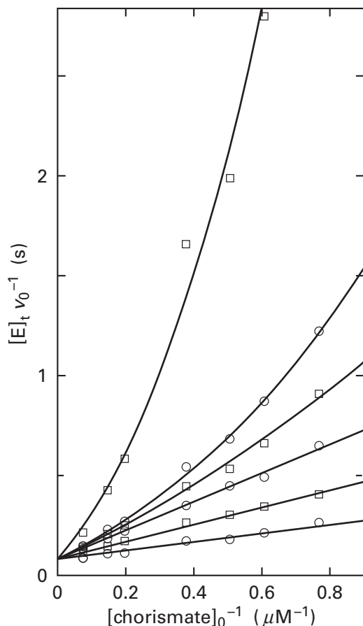
Figure 6-18: Competitive heterotropic allosteric inhibition of anthranilate synthase from S. typhimurium by L-tryptophan. 104,105 Solutions contained 20 mM L-glutamine, 10 mM MgCl, various concentrations of chorismate, various concentrations of L-tryptophan, and 0.1 M potassium phosphate at pH 7.0 and 25 °C. The reaction was initiated by adding anthranilate synthase, and the rate of production of anthranilate was followed fluorometrically ( \lambda_{\text{ex}} = 308 \text{ nm} ; \lambda_{\text{em}} = 388 \text{ nm} ) over the first few minutes to obtain initial rates. The initial rates were converted to unit of second -1 . The reciprocal of each initial rate ( v_0^{-1} in seconds) is plotted as a function of the respective reciprocal of the initial concentration of chorismate (micromolar -1 ) at six fixed concentrations of L-tryptophan: in ascending order of the curves, 0, 2.5, 5.0, 7.5, 10, and 20 \mu\text{M} . The lines and curves are drawn by hand.
