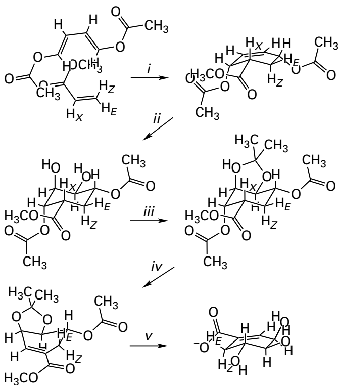
Figure 4-30: Synthesis of D-shikimate from methyl acrylate and trans,trans -1,4-diacetoxy-1,3-butadiene. 511,512 (i) The diene and dienophile were condensed in anhydrous xylene at reflux in a Diels-Alder cycloaddition that proceeded with the usual stereochemical consequences. In the direction of approach shown, methyl acrylate is below the diene. The two inwardly directed hydrogens on the diene are pushed upward, and the two outwardly directed acetoxy groups respond by rotating downward. The Z -hydrogen and the methoxycarbonyl group of the dienophile are pushed downward, and the E -hydrogen and the X -hydrogen respond by rotating upward to give the enantiomer drawn. The other enantiomer of the endo product is produced when the dienophile approaches from the top of the diene. (ii) Osmium tetroxide in tetrahydrofuran/pyridine was used to perform a cis -hydroxylation of the carbon-carbon double bond. The hydroxylation proceeded trans to the two adjacent acetoxy groups because of their bulk and the bulk of the osmium tetroxide. (iii) The two vicinal cis -hydroxy groups were incorporated into an acetal with anhydrous acetone under a stream of hydrochloric acid. (iv) The elimination of acetic acid by concerted loss of the acidic hydron, H_X^+ , and the good leaving group, CH_3COO^- , was accomplished by pyrolysis in a sealed tube at 285 °C. (v) The acetal and the two esters were hydrolyzed in 60% acetic acid to yield racemic shikimic acid. The D-enantiomer of shikimate was isolated as the crystalline salt with (-)-1-amino-1-phenylethane.
