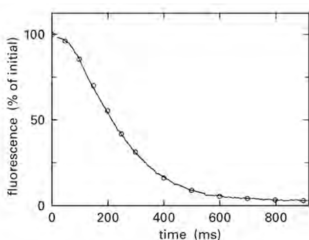
Figure 5-37: Lag in oxidation of NADPH when the complex between NADPH and the fatty-acid synthase system is mixed with acetyl-SCoA and malonyl-SCoA. 963 A solution containing the fatty-acid synthase system from G. gallus (4.3 \mu\text{M} in active sites) and 1.5 \mu\text{M} NADPH was mixed with a solution of 110 \mu\text{M} acetyl-SCoA and 200 \mu\text{M} malonyl-SCoA in an apparatus for stopped flow (dead time 2 ms). The two solutions were buffered at pH 7.0 with 0.1 M potassium phosphate at 25 °C. Fluorescence of the solution in the observation chamber at wavelengths greater than 420 nm ( \lambda_{\text{excitation}} = 367 \text{ nm} ), which was due to NADPH, was monitored as a function of time (milliseconds). The solid trace is the direct observation of fluorescence as a percentage of the initial reading, and the open circles are values calculated by Equation 5-376 with k_1 = 4.3 \text{ s}^{-1} , k_2 = 9.5 \text{ s}^{-1} , and [\text{NADPH}]_0 = 100\% . It was necessary to add a background of 18% to all calculated values to obtain a satisfactory fit. Adapted with permission from reference 963. Copyright 1983 American Chemical Society. https://doi.org/10.1021/bi00295a037
