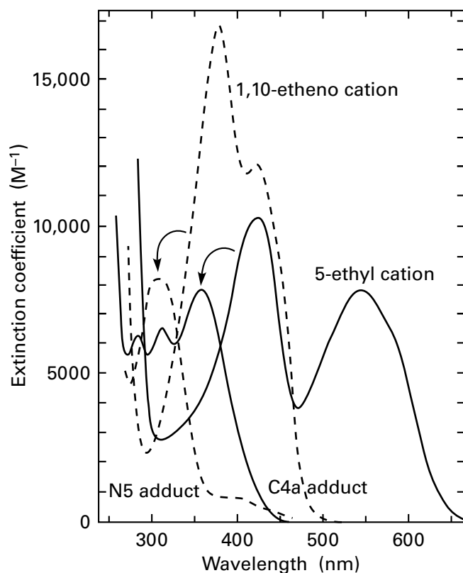
Figure 2-16: Absorption spectra of adducts to oxidized flavin. The spectrum 373 for the adduct of sulfite to nitrogen 5 (N5 adduct) of 7,8-dimethyl-1,10-ethenoisalloxazininium (Equation 2-124) was obtained by adding sufficient \text{NaHSO}_3 to a 40 \mu\text{M} aqueous solution of 7,8-dimethyl-1,10-ethenoisalloxazininium perchlorate at pH 7 to convert all of the isoalloxazininium to the adduct of sulfite at nitrogen 5. The spectrum of 7,8-dimethyl-1,10-ethenoisalloxazininium (1,10-etheno cation) in the same solution was taken before the sulfite was added. The strong absorbance of the isoalloxazininium between 350 and 500 nm disappeared as the sulfite adduct formed. The spectrum 374 for the adduct of ethoxide to carbon 4a (C4a adduct) of 3,7,8,10-tetramethyl-5-ethylisalloxazininium ion (Equation 2-128) was obtained by dissolving 3,7,8,10-tetramethyl-5-ethylisalloxazininium perchlorate in ethanol. The spectrum 375 of the initial 3,7,8,10-tetramethyl-5-ethylisalloxazininium ion (5-ethyl cation) was obtained by dissolving 3,7,8,10-tetramethyl-5-ethylisalloxazininium perchlorate in 0.1 M sodium perchlorate at pH 3.
