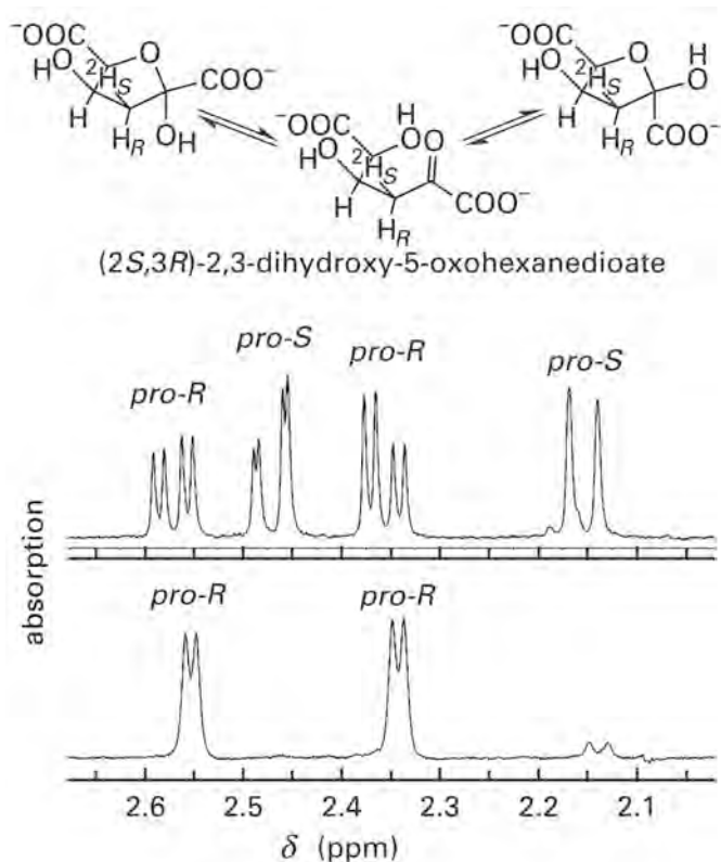
Figure 4–28: Determination of the prochiral stereochemistry of the reaction catalyzed by galactarate dehydratase ( D - threo -forming) from A. tumefaciens . 468 Portions (those between 2.7 and 2.0 ppm) of two proton nuclear magnetic resonance spectra of different samples of (2 S ,3 R )-2,3-dihydroxy-5-oxohexanedioate, the product of the enzymatic reaction when meso -galactarate is the reactant, are shown. These portions of the spectra contain the absorptions from the two protons on carbon 4 in the two furano anomers of (2 S ,3 R )-2,3-dihydroxy-5-oxohexanedioate present at equilibrium in the solution. The (2 S ,3 R )-2,3-dihydroxy-5-oxohexanedioate that gave the upper spectrum was obtained when meso -galactarate was dehydrated by galactarate dehydratase ( D - threo -forming) in 1 H 2 O. Absorptions from both the 4- pro-S and the 4- pro-R hydrons in (2 S ,3 R )-2,3-dihydroxy-5-oxohexanedioate are observed. These assignments for the spectra of the anomers were made from the respective magnitudes of the vicinal C3–C4 1 H– 1 H coupling constants, 1 H– 13 C heteronuclear single quantum coherence nuclear Overhauser effects, and 13 C nuclear magnetic resonance spectra. The respective absorptions are split by the other hydrogen on carbon 4 and the hydrogen on carbon 3 into doublets of doublets. Dehydration of meso -galactarate by the enzyme was then performed in 2 H 2 O so that the hydrogen on prochiral carbon 4 that was added by the enzyme in place of the hydroxy group removed during the dehydration (Equation 4–227) would be a deuterium. The absorption from the 4- pro-S proton was missing from the spectrum (lower two panels) of the deuterated product, and the vicinal splitting of the 4- pro-R proton by the 4- pro-S hydrogen was also missing from the absorption of the 3- pro-R proton. These observations demonstrate that the hydron added by the enzyme to carbon 4 is the 4- pro-S hydrogen from (2 S ,3 R )-2,3-dihydroxy-5-oxohexanedioate. Adapted with permission from reference 468. Copyright 2014 American Chemical Society. https://pubs.acs.org/doi/10.1021/bi5005377
