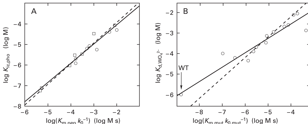
Figure 3–30: (A) Correlation between the dissociation constants, K_{i,c,pho} , for a set of phosphonates from the active site of bovine carboxypeptidase A and the values of the steady-state rate constants, K_{m,pep} k_0^{-1} , for the homologous reactants. 213 The reactants, listed in order of increasing values for K_{m,pep} k_0^{-1} , were the peptides Cbz-Phe-Ala-Ala, Cbz-Ala-Ala-Ala, Cbz-D-Ala-Ala-Ala, Cbz-Leu-Ala-Ala-Ala, Cbz-Phe-Ala-Ala-Ala, Cbz-Gly-Ala-Ala, Pp-Ala-Ala-Ala, Pp-Ala-Ala-Ala-Ala, Cbz-Ala-Ala-Ala-Ala, Ac-Ala-Ala-Ala-Ala, Ac-Ala-Ala-Ala, Cbz-Ala-D-Ala-Ala-Ala, Ac-Ala-D-Ala-Ala-Ala, and Ac-D-Ala-Ala-Ala, where Cbz is benzyloxycarbonyl, Pp is 3-phenylpropanoyl, and Ac is acetyl. In each case, the peptide is cleaved by the enzyme at the peptide bond in the carboxy-terminal alanylalanine. An analogue of each peptide was synthesized in which a phosphonate (3–73) replaced the peptide bond between the carboxy-terminal alanylalanine as the phosphonamidate replaces the peptide bond in analogue 3–83. Each analogue was assayed for its ability to inhibit carboxypeptidase A at pH 7.6, 27 °C, and an ionic strength of 0.5 M with the fluorescent reactant N -[3-(2-furyl)acryloyl]-L-phenylalanyl-L-phenylalanine. The analogues were all competitive inhibitors of the enzyme. The common logarithms of the competitive inhibition constants, K_{i,c,pho} (molar), for tripeptides (□) and tetrapeptides (○) are plotted as a function of the common logarithms of their respective steady-state
