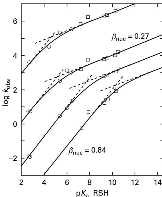
Figure 1-11: Brønsted correlations between the rate constants for nucleophilic substitutions at four different acetate esters by a series of nucleophilic aryl thiolate ions ( \circ ) and alkyl thiolate ions ( \square ), the conjugate acids of which have different acid dissociation constants. 141 The rates for each nucleophilic substitution (Equation 1-50) were followed at two or more values of pH at an ionic strength of 1.0 M and at 25 °C. The values of pH chosen in each case were those appropriate to the \text{p}K_{\text{a}} of the particular thiol the thiolate ion of which was used as the nucleophile. The pH at which each rate was measured was used to determine the actual concentration of thiolate ion in the solution. For each of the 36 combinations of electrophile and thiolate ion, represented by the 36 points on the graph, the rate constants calculated, based on the actual concentration of thiolate ion, were the same for all values of pH. The common logarithms of the observed rate constants are plotted as a function of the values of the \text{p}K_{\text{a}} for the thiol. The thiols chosen, in order of increasing \text{p}K_{\text{a}} , were pentafluorobenzenethiol ( \text{p}K_{\text{a}} = 2.68 ), 2,3,5,6-tetrafluorobenzenethiol ( \text{p}K_{\text{a}} = 2.75 ), 4-nitrobenzenethiol ( \text{p}K_{\text{a}} = 4.5 ), 3,4-dichlorobenzenethiol ( \text{p}K_{\text{a}} = 5.48 ), 4-acetamidobenzenethiol ( \text{p}K_{\text{a}} = 6.08 ), benzenethiol ( \text{p}K_{\text{a}} = 6.43 ), 2,2,2-trifluoro-1-sulfanylethane ( \text{p}K_{\text{a}} = 7.30 ), methyl 2-sulfanylacetate ( \text{p}K_{\text{a}} = 7.91 ), methyl 3-sulfanylpropionate ( \text{p}K_{\text{a}} = 9.33 ), 2-sulfanylethanol ( \text{p}K_{\text{a}} = 9.61 ), sulfanylethane ( \text{p}K_{\text{a}} = 10.35 ), and 1-sulfanylpropane ( \text{p}K_{\text{a}} = 10.53 ). Each of the four curves in the figure is for the nucleophilic substitutions of a particular acetate ester. The four acetate esters used as electrophiles, in descending order on the field of the graph, were 1-acetoxy-4-methoxypyridinium ion, 2,4-dinitrophenyl acetate, 4-nitrophenyl acetate, and phenyl acetate. The products produced by the leaving groups were 4-methoxypyridine 1-oxide, 2,4-dinitrophenolate ion, 4-nitrophenolate ion, and phenolate ion, respectively. The curves drawn through the data each have linear asymptotes of the same slope to the left and of the same slope to the right of the respective inflections. The slopes of the linear asymptotes, the values of \beta_{\text{nuc}} , are 0.84 to the left and 0.27 to the right. There is a gradual change in slope in the middle of each curve.
