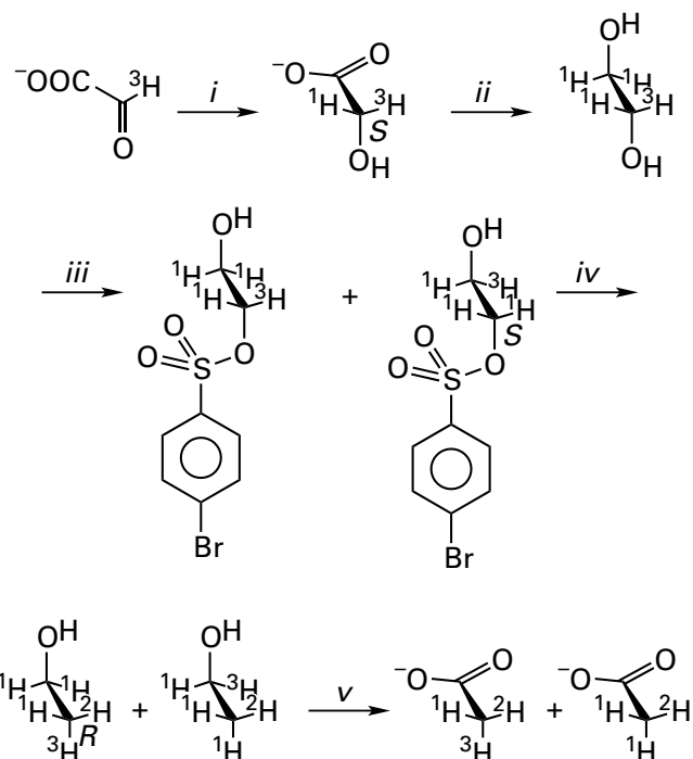
Figure 4–31: Synthesis of chiral acetate from [2\text{-}^3\text{H}] glyoxylate. 564 (i) [2\text{-}^3\text{H}] Glyoxylate was reduced with NADH and L-lactate dehydrogenase to produce ( S )- [2\text{-}^3\text{H}] glycolate. (ii) The methyl ester of ( S )- [2\text{-}^3\text{H}] glycolate was reduced chemically with \text{LiAlH}_4 to produce ( S )- [1\text{-}^3\text{H}] ethylene glycol. (iii) An equimolar mixture of the two 4-bromobenzenesulfonates (brosylates) of the labeled ethylene glycol was produced by sulfonation with 4-bromobenzenesulfonyl chloride. (iv) The leaving ability of a 4-bromobenzenesulfonyl group was exploited to promote reduction of the two regioisomers with [^2\text{H}]\text{LiAlH}_4 by substitution with deuteride with inversion of configuration. (v) The resulting equimolar mixture of ( 2R )- [2,2\text{-}^2\text{H},^3\text{H}] ethanol and ( 1S )-1-tritio-2-deuterioethanol was oxidized with \text{O}_2 over a platinum catalyst, producing a mixture of ( R )- [^2\text{H},^3\text{H}] acetate and [^2\text{H}_1] acetate. Because only a portion of the original [2\text{-}^3\text{H}] glyoxylate was actually tritiated, the only effect of the equimolar yield of [^2\text{H}_1] acetate was to halve the specific radioactivity of the product relative to that of the initial [2\text{-}^3\text{H}] glyoxylate, not to introduce a species of acetate that was not already unavoidably present.
