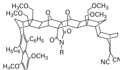
2–76 R = p -ethylphenyl 2–77 R = propyl
