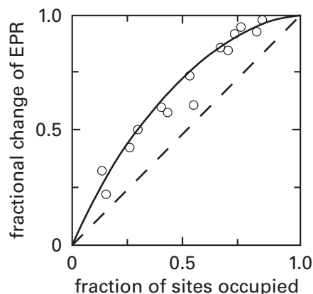
Figure 6–15: Plot of the extent of conformational change 68 of spin-labeled glycogen phosphorylase a from O. cuniculus as a function of the fraction of sites occupied by the heterotropic allosteric effector AMP 2- . Phosphorylase a was modified with N -(1-oxyl-2,2,6,6-tetramethyl-4-piperidinyl)iodoacetamide to introduce one stable nitroxyl radical into each subunit of the protein. Binding of AMP 2- was followed by equilibrium dialysis by measuring at equilibrium the molar concentrations of [U- 14 C]adenosine 5'-monophosphate in the two chambers, one containing 4 \mu M phosphorylase a and one lacking phosphorylase a , for a series of concentrations of the ligand. The binding displayed positive deviation from ideal behavior and could be fit with Equation 6–35 with L_0 = 3 , K_{dAMP} = 2 \mu M, K'_{dAMP} = 10 \mu M, and n = 4 . As the occupation of the enzyme by AMP 2- was increased by increasing the free concentration of the ligand, the electron paramagnetic resonance (EPR) spectrum changed as the result of broadening of the outer two absorbances of the triplet. The binding of AMP 2- was measured and the electron paramagnetic resonance spectra were recorded for a series of samples with the same free concentrations of AMP 2- . For each free concentration of AMP 2- , the broadening of the spectra observed at that concentration, as a fraction of the broadening observed at saturation with AMP 2- [O; fractional change of EPR], is plotted as a function of the respective fraction of sites for AMP 2- that were occupied at the same free concentrations of AMP 2- . The solid curve is not a fit to the data. It is instead the curve for the function of Equation 6–49 using values for the fraction of the enzyme in the R conformation calculated with Equation 6–48 with L_0 = 3 , K_{dAMP} = 2 \mu M, K'_{dAMP} = 10 \mu M, and n = 4 that were established from the binding of [U- 14 C]adenosine 5'-monophosphate to the enzyme.
