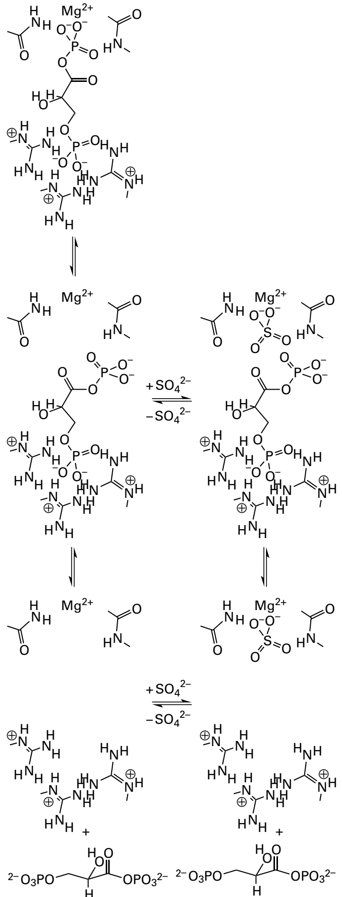
Figure 3-62: Effect of sulfate on the enzymatic activity of yeast phosphoglycerate kinase. 1156 Samples were prepared that contained phosphoglycerate kinase in 5 \mu\text{M} ( \bullet ), 50 \mu\text{M} ( \circ ), 0.5 mM ( \square ), 1.5 mM ( \triangle ), or 5.0 mM ( \nabla ) \text{MgATP}^{2-} and 1.0 mM free \text{Mg}^{2+} , 50 mM 3-phosphoglycerate, and various concentrations of \text{Na}_2\text{SO}_4 . The initial rate of production of 1,3-bisphosphoglycerate was monitored by the decrease in concentration of NADH in a coupled assay involving glyceraldehyde-3-phosphate dehydrogenase, creatine kinase, creatine phosphate, and triose-phosphate isomerase. Initial rates of decrease in the fluorescence of NADH were measured continuously for each sample. The activity of the enzyme (percent of the initial rate in the absence of phosphate) is presented as a function of the concentration of \text{Na}_2\text{SO}_4 (millimolar).
