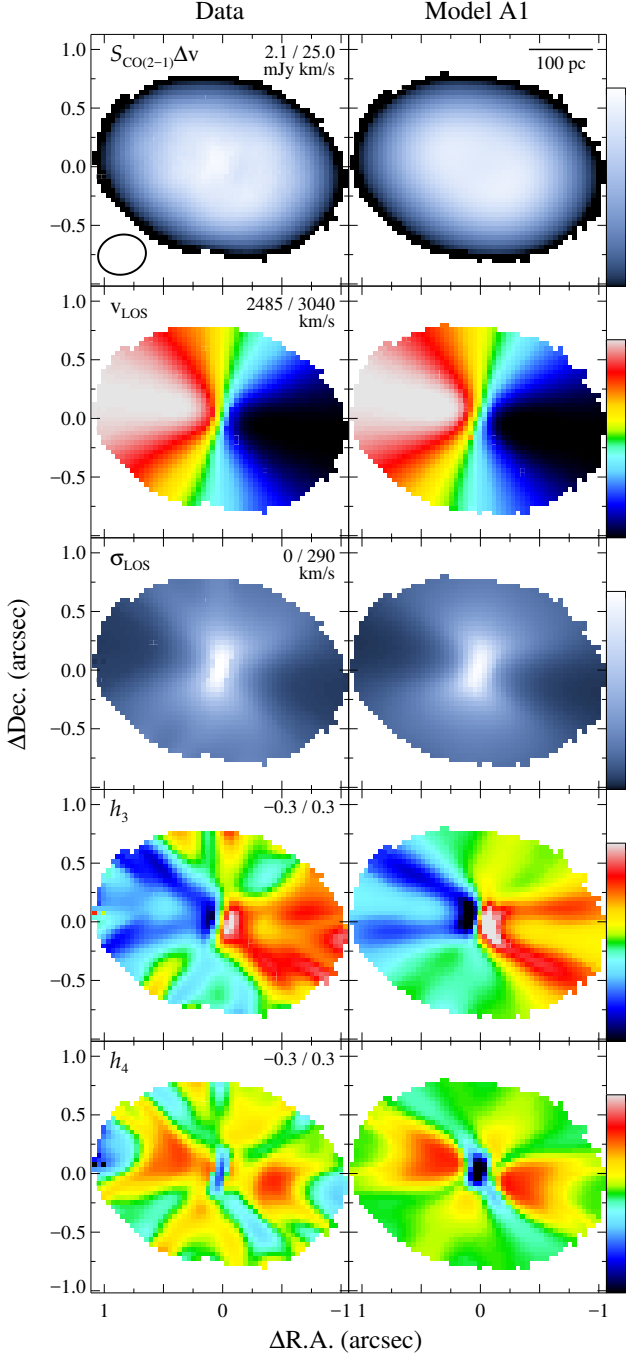
Figure 15. Comparison between flux and kinematic moments measured from the Cycle 2 CO(2–1) data cube ( left ) and those measured from the best-fitting model A1 ( right ). Ranges in each data frame indicate the intensity/color scale extremes. Due to strong central beam smearing of this \sim 0''.44 -resolution data, the kinematic signature of the BH is primarily found in higher-order (especially h_3 ) moments.
