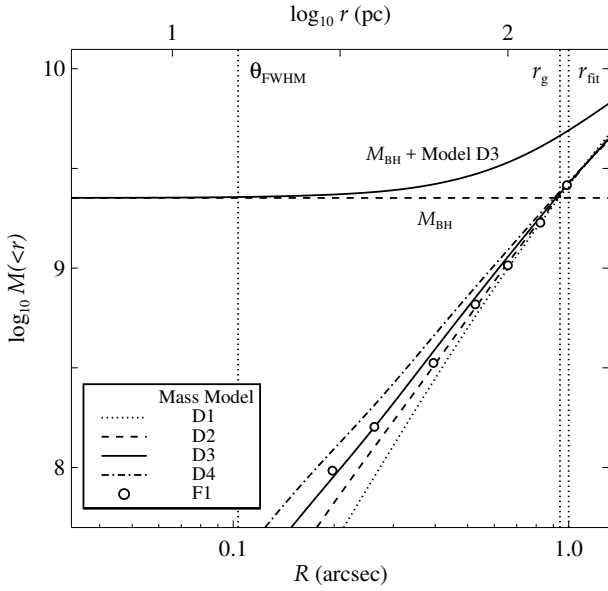
Figure 22. Enclosed mass M(<r) = rv_c^2/G in NGC 3258 as a function of physical radius for the various MGE galaxy mass distributions (with the corresponding v_c^* values scaled by best-fit \sqrt{\Upsilon_H} ; see Tables 2 and 3) that are extrapolated beyond the edge of the CO rotation pattern. Dotted vertical lines indicate the ALMA Cycle 4 average beam size \theta_{\text{FWHM}} and fitting region radius r_{\text{fit}} , with r_g = 0''.94 determined for a BH mass of 2.249 \times 10^9 M_\odot .
