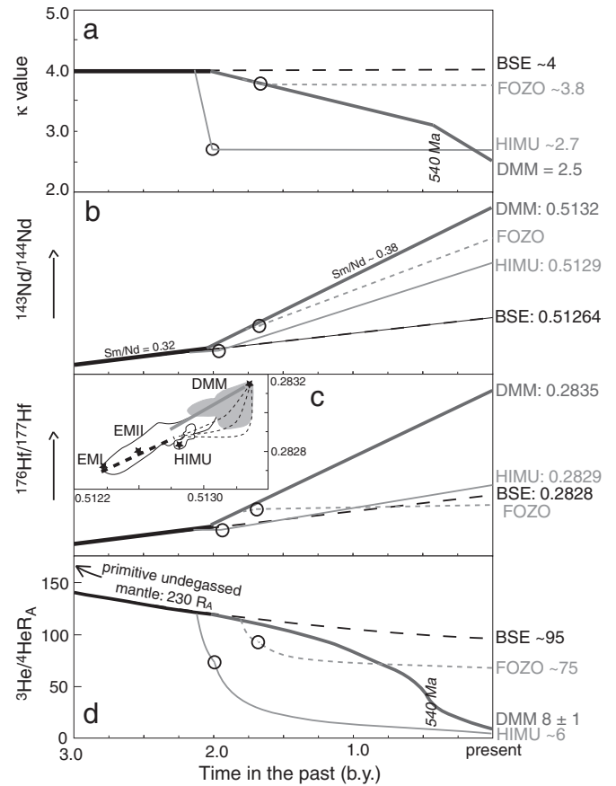
Fig. 6. Schematic evolution diagrams for the different chemical/isotopic systems discussed in the text. a) Modified post-Archaean uranium recycling (PURE) model ( Elliott et al., 1999 ). HIMU \kappa value was calculated using a 0.7128 slope of the Mangaia ^{208}\text{Pb}/^{204}\text{Pb} – ^{206}\text{Pb}/^{204}\text{Pb} array and 3.2 Ga ^{207}\text{Pb}/^{206}\text{Pb} isochron age (from Fig. 4). b) Idealized ^{143}\text{Nd}/^{144}\text{Nd} evolution; not to scale to emphasize the modern separations among DMM, FOZO, HIMU, and BSE. c) Idealized ^{176}\text{Hf}/^{177}\text{Hf} evolution; also not to scale to emphasize the modern separations among DMM, FOZO, HIMU, and BSE. The global correlation between ^{143}\text{Nd}/^{144}\text{Nd} and ^{176}\text{Hf}/^{177}\text{Hf} is summarized in the inset figure. White field represents OIB whereas gray field represents MORB. d) Modified ^3\text{He}/^4\text{He}_{\text{RA}} evolution model of Class and Goldstein (2005) . In all diagrams, circles in HIMU and FOZO lines represent time of subduction. See text for more detailed discussions.
