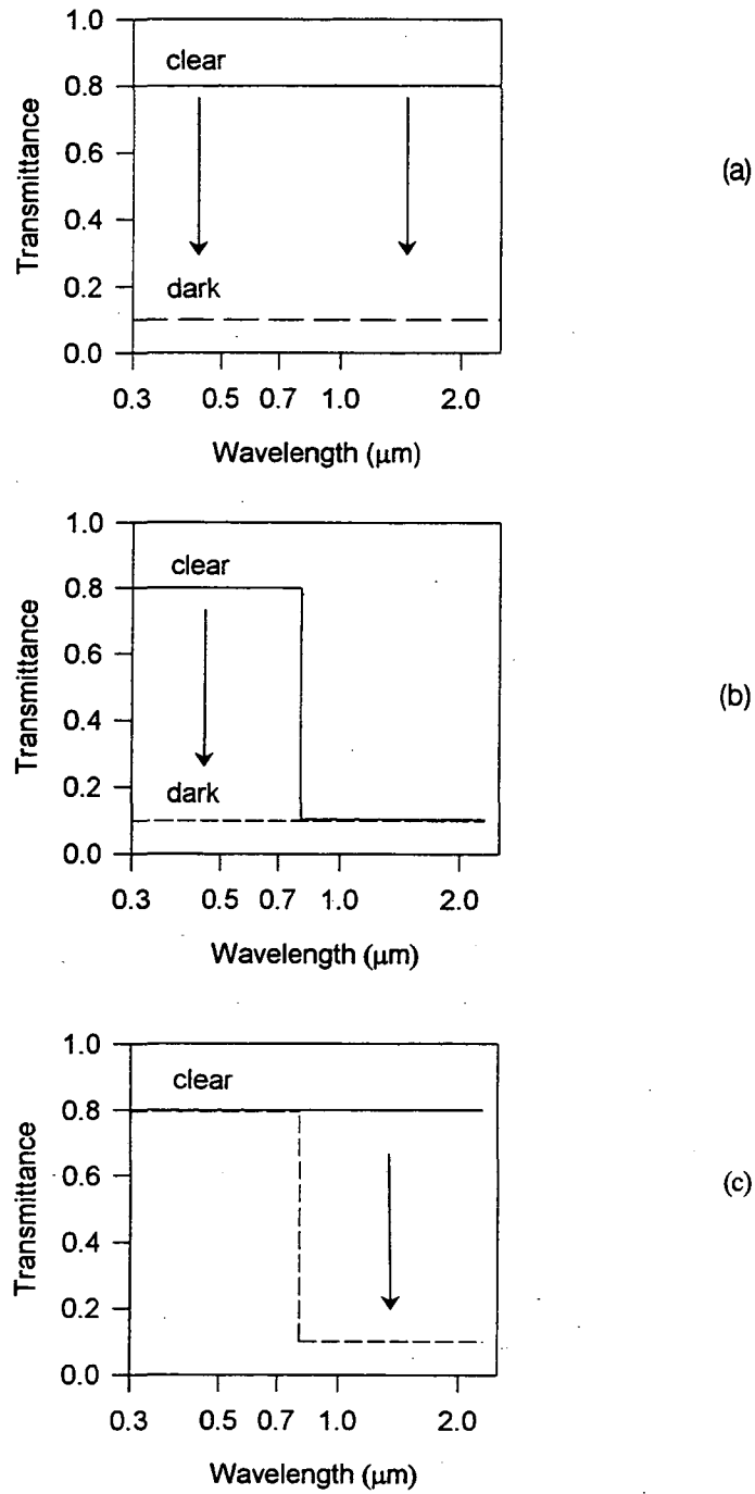
Fig. 1. Idealized electrochromic spectra in the "clear" and "darkened" state: (a) uniform switching occurs over the entire solar spectrum; (b) switching occurs over the visible spectrum only with constant low transmission in the near infrared in both "clear" and "dark" states; and (c) switching occurs over the infrared spectrum only with constant high transmission in the visible spectrum in both "clear" and "dark" states.
