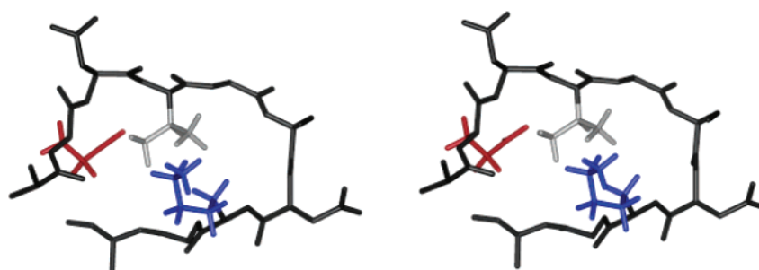
FIGURE 1. Stereoviews of NMR-derived structural models of A\beta(21-30) . Heavy-atom representations are shown with Glu22 (red), Val24 (gray), and Lys28 (blue) highlighted. Other atoms are black. All structures display a main chain turn at Val24–Lys28 and a relatively ordered N-terminus. The two families differ in the orientation of the Lys28 side chain.
