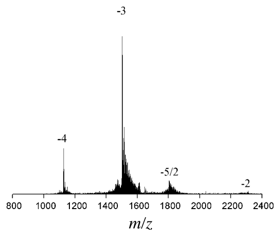
FIGURE 2. Negative ion mass spectrum of A\beta_{42} . The z/n values of the peaks are indicated.
