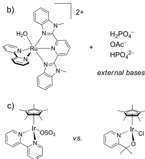
Figure 2. Water-oxidation catalysts previously investigated for base-assisted substrate deprotonation as described in the literature. [8–11]
