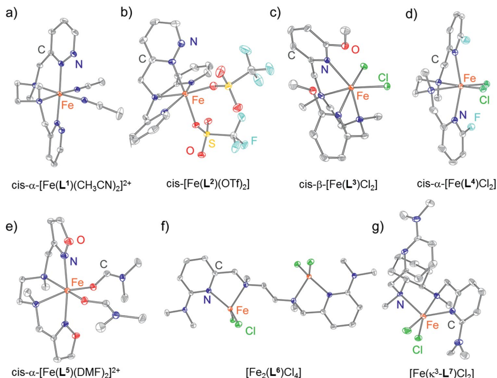
Figure 4. Thermal ellipsoid plots of the structures of the \text{Fe}^{\text{II}} complexes in (a) [\text{Fe}(\text{L}^1)(\text{CH}_3\text{CN})_2]^{2+} , (b) [\text{Fe}(\text{L}^2)(\text{OTf})_2] , (c) [\text{Fe}(\text{L}^3)\text{Cl}_2] , (d) [\text{Fe}(\text{L}^4)\text{Cl}_2] , (e) [\text{Fe}(\text{L}^5)(\text{dmf})_2]^{2+} , (f) [\text{Fe}_2(\text{L}^6)\text{Cl}_4] , and (g) [\text{Fe}(\text{L}^7)\text{Cl}_2] with thermal ellipsoids rendered at 40% probability. Orange, blue, gray, red, green, cyan, and yellow ellipsoids correspond to iron, nitrogen, carbon, oxygen, chlorine, fluorine, and sulfur atoms, respectively. Hydrogen atoms, uncoordinated counterions, and solvents have been omitted for clarity.
