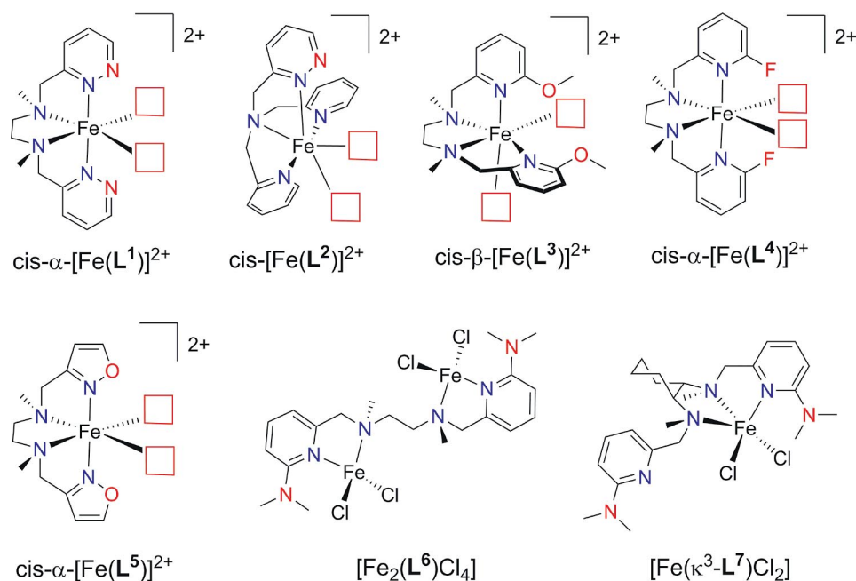
Figure 3. Schematic representations of the prepared \text{Fe}^{\text{II}} complexes. Red boxes correspond to labile coordination sites that are occupied either by solvent molecules or anionic ligands.
