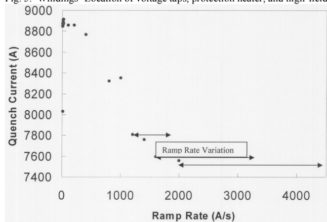
Fig. 6. Quench Current versus Ramp Rate & variation shown for TAMU2.
