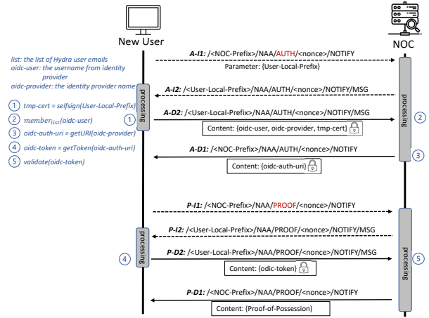
Figure 6: User authentication workflow
