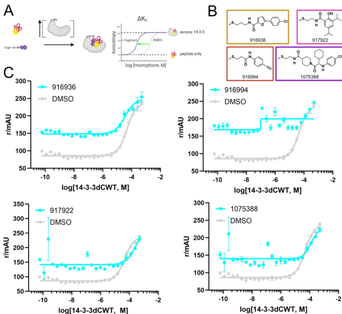
Figure 2.5. Overview of protein titration experiments. (A) Outline of protein titration process. 2 mM fragment is incubated with fluorescently labeled procaspase-2 phospho-peptide and 14-3- \sigma is titrated from high concentration to low concentration. If the compound is a stabilizer, a shift in K_D to the left of the DMSO control indicates cooperativity between the fragment, protein, and phospho-peptide. (B) Chemical structures of the four highlighted compounds. (C) Protein titration curves of 916936 (top left), 916994 (top right), 917922 (bottom left), and 1075388 (bottom right). Cyan curves indicate incubation with 2 mM fragment. Grey curves are DMSO controls.
