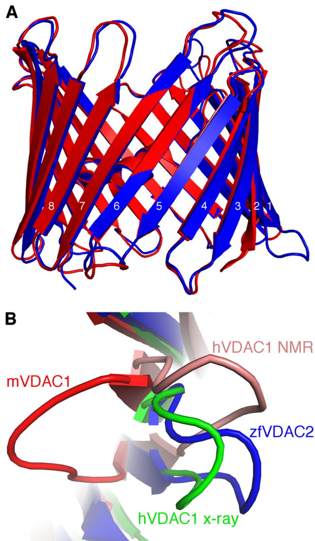
FIGURE 4. Superposition of zfVDAC2 and VDAC1. A, zfVDAC2 in blue and mVDAC1 (Protein Data Bank code 3EMN) in red were aligned with a C_{\alpha} root mean square deviation of 0.98 Å. There is a large displacement ( \sim 12 Å) in the loop between \beta -strands 1 and 2. B, an IMS view of the loop between \beta -strands 1 and 2, including zfVDAC2 in blue, mVDAC1 in red, hVDAC1 (Protein Data Bank code 2JK4) in green, and a representative NMR conformer of hVDAC1 (Protein Data Bank code 2K4T) in salmon.
