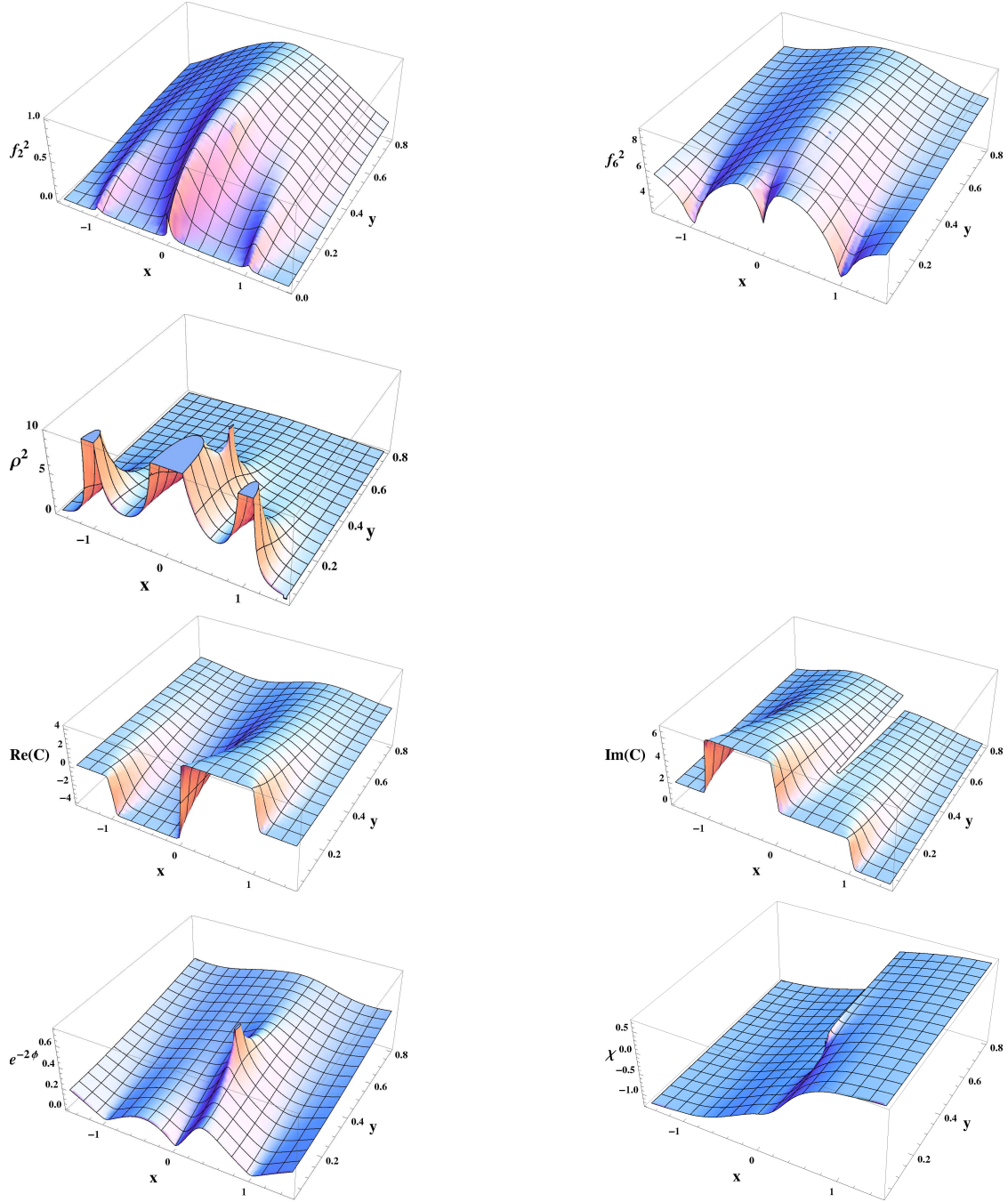
Figure 4: The metric factors f_2^2 , f_6^2 and \rho^2 , the real and imaginary parts of the two-form potential \mathcal{C} and axion and dilaton for the 3-pole solution with [1, 0] branch point.
