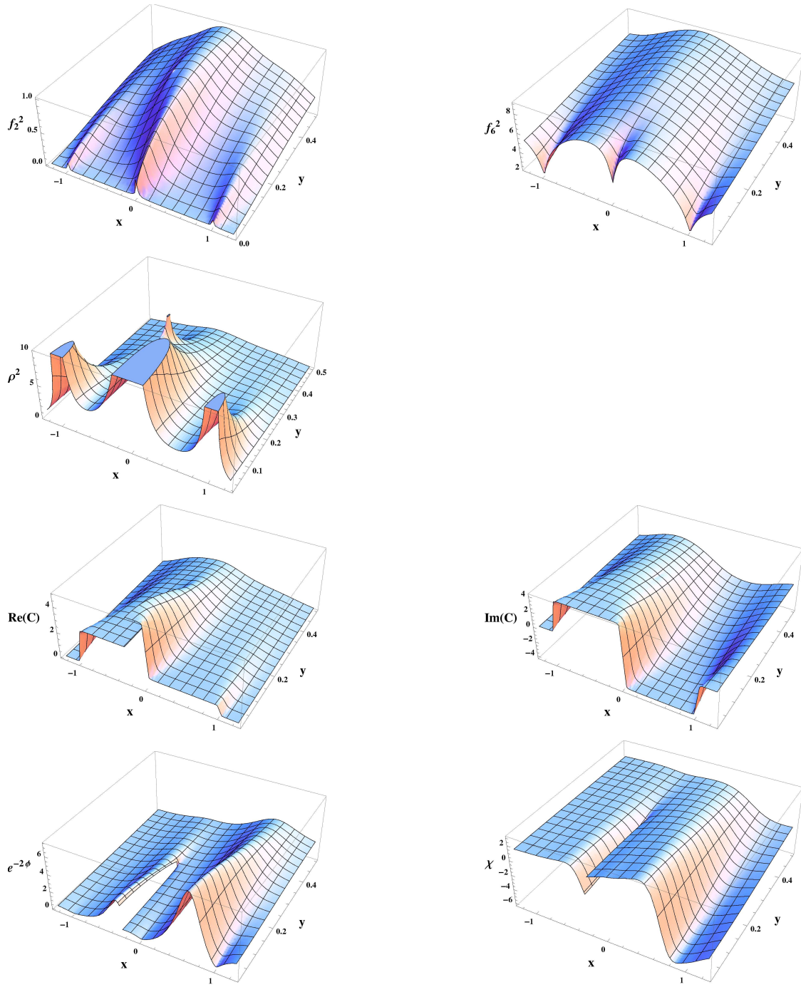
Figure 5: The metric factors f_2^2, f_6^2 and \rho^2 , the real and imaginary parts of the two-form potential C and axion and dilaton for the 3-pole solution with [0, 1] monodromy.
