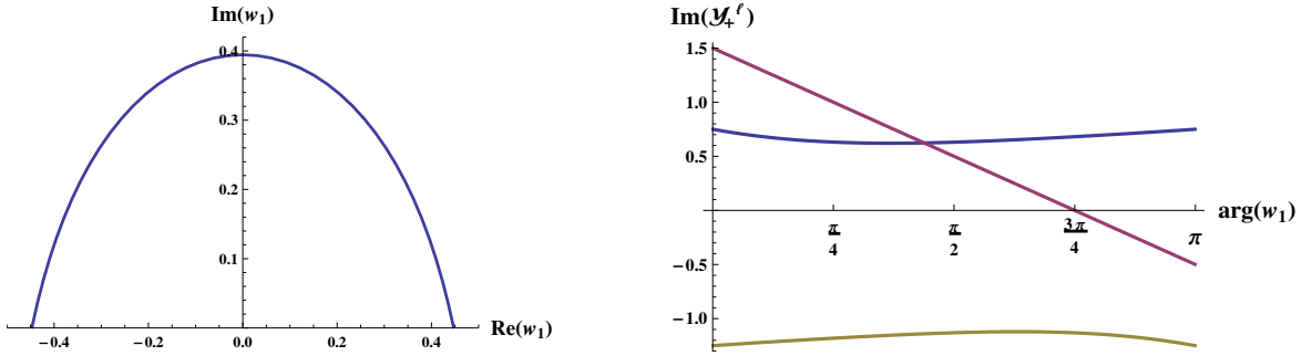
Figure 3: On the left hand side the allowed locations for the branch point w_1 in the upper half plane, for the solution (4.7) with a single puncture corresponding to a D7-brane and n_1 = 1 . On the right hand side the imaginary part of the charges along the curve shown on the left. At \text{arg}(w_1) = \pi the curves are, from top to bottom, \text{Im}(\mathcal{Y}_+^1) , \text{Im}(\mathcal{Y}_+^2) and \text{Im}(\mathcal{Y}_+^3) .
