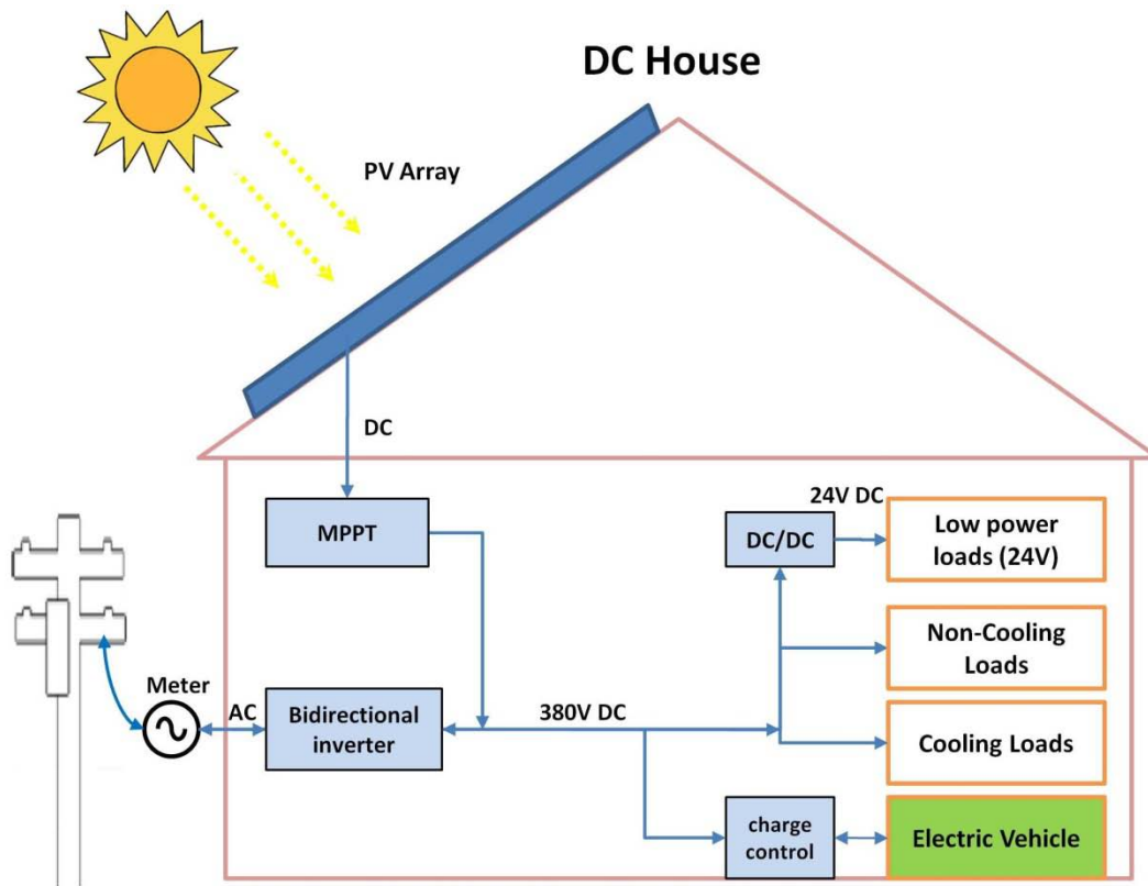
Figure 3. Direct-DC Power System.
