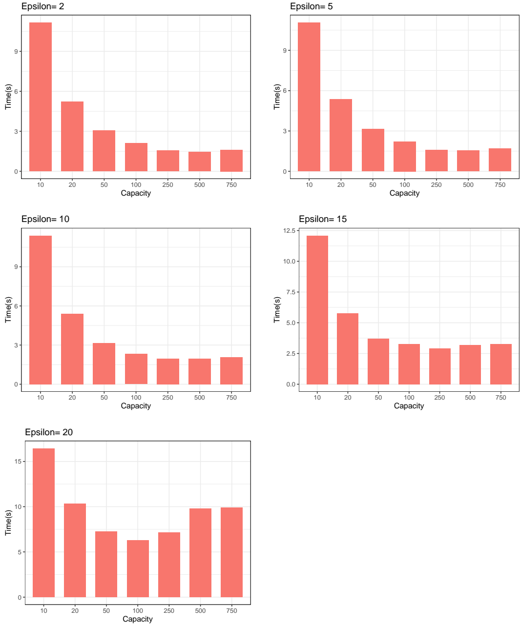
Figure 4.14: Execution time testing different values for Capacity ( c ) and Epsilon ( \epsilon ).
