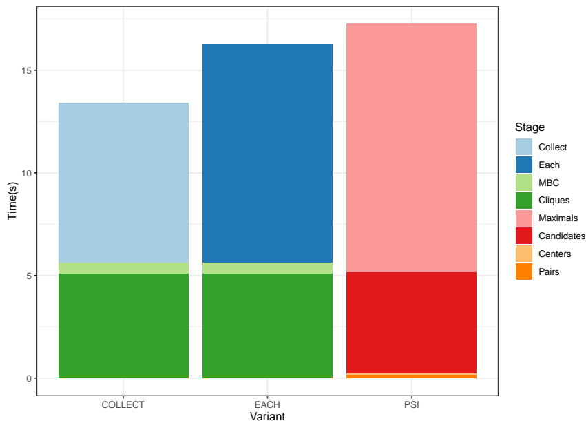
Figure 4.20: Execution time of the two variants of CMBC approach compared to standard PSI in the partition 187 with \approx 2K points present ( \epsilon = 20m ).
