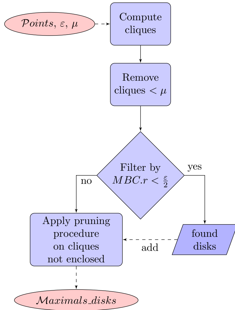
Figure C.1: Schematic description of the Clique and MBC approach.
