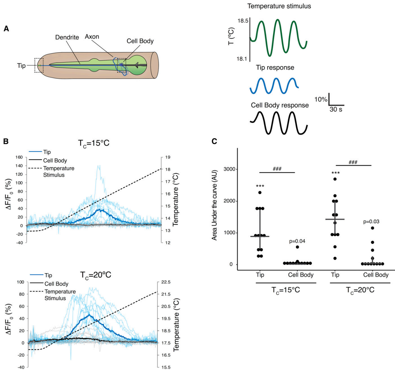
Figure 3 FlincG3 fluorescence at AFD thermosensory neuron endings changes in response to a rising temperature ramp in an experience-dependent manner. (A) (Left) Cartoon of the bilateral AFD thermosensory neurons in the head of C. elegans (adapted from www.wormatlas.org ). Dashed boxes indicate regions in which imaging of FlincG3 fluorescence was performed. (Right) Schematic of oscillating temperature stimulus (green lines) and changes in intracellular calcium at the AFD sensory tips (blue lines) and cell bodies (black lines) measured via changes in fluorescence of the cameleon calcium sensor expressed in AFD (adapted from Clark et al. (2006)). (B) Changes in FlincG3 fluorescence at the tips (blue traces) and cell bodies (gray traces) of AFD neurons in response to a rising linear temperature ramp (black dashed lines). The slope of the ramp was 0.02^\circ per second. Bolded blue and black traces indicate the average response, thinner traces indicate responses of individual neurons. Animals were cultivated overnight at temperature ( T_c ) of 15^\circ (top) or 20^\circ (bottom). n = 12 animals for each T_c . (C) Area under the curve measurements of the AFD neuron tip are different from measurements of the cell body. Horizontal bars indicate mean area under the curve, top and bottom of vertical bar indicates upper and lower quartile, respectively. *** indicates mean different from 0 at P < 0.0001 (mean P -value from bootstrap t -test). ### indicates tip different from cell body at P < 0.001 (two sample t -test).
