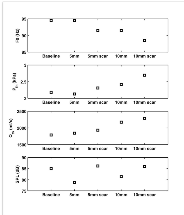
Figure 2. The onset phonatory frequency ( F_0 ), phonation threshold pressure ( P_{th} ), threshold flow rate ( Q_{th} ), and outside sound pressure level (SPL) is displayed as functions of the extent of cordectomy in the physical model.
