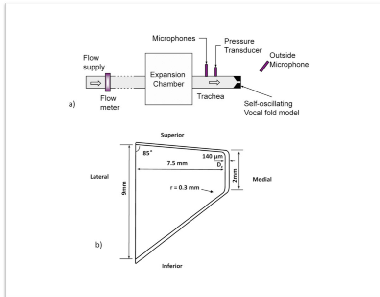
Figure 1. Sketch of (a) the experimental setup and (b) the coronal cross-sectional geometry of the two-layer physical model.
