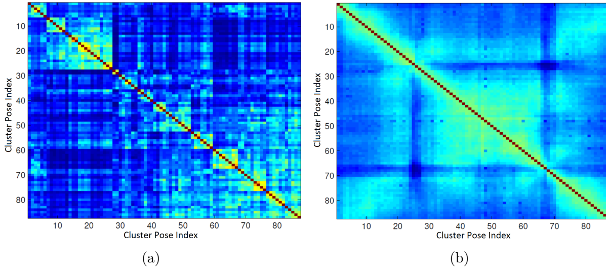
Figure 3.8: Optimization of the correlation matrix used in clustering. (a): The correlation matrix of a cluster before optimization of pairwise constraints. (b): The correlation matrix after FICP has been run on the pairwise constraints.
