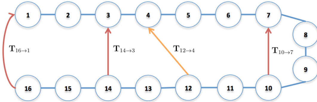
Figure 4.25: An illustrative example of manual loop closure re-optimization. When the manual loop closure, denoted in orange, is processed.
