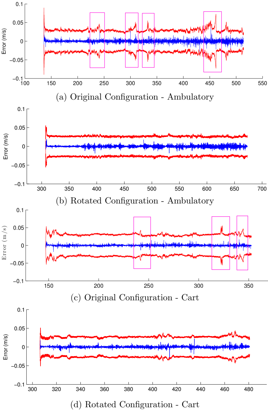
Figure 4.35: Comparison of the variance of the forward direction of the system’s velocity for the different laser configurations. The blue lines indicate the estimates of the error state while the red lines denote the 3\sigma bounds on the error estimate. Pink boxes indicate degenerate locations. (a): The variance plot for the original configuration when human mounted. Notice the regions of the dataset where degeneracies caused rapid increase in the velocity’s variance. (b): The variance plot using the rotated laser configuration when human mounted. (c): The variance plot after mounting the system on a cart using the normal configuration. (d): The variance plots for the rotated laser configuration and mounting the system on a cart.
