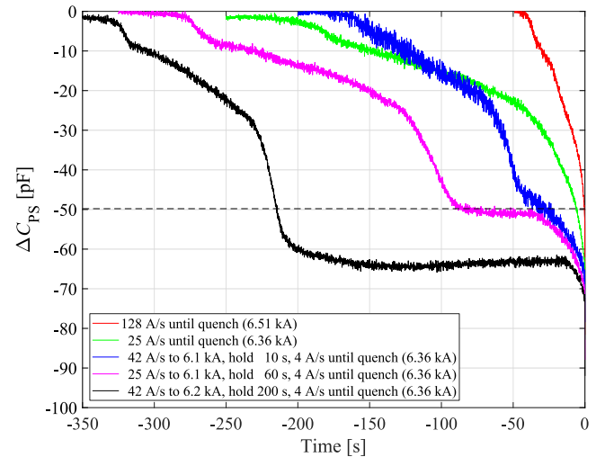
Figure 11. Thermal runaway detection in RC3 coil in liquid helium at T_{\text{bath}} = 4.2 K, using the proposed stray-capacitance monitoring system. Measured P-S capacitance change versus time. The proposed detection threshold \Delta C_{\text{threshold}} is indicated with a black dashed line. Quenches occurred while submitting I_m to different transients, which are described in the legend.
