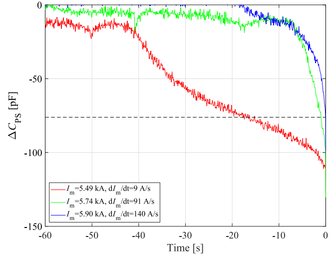
Figure 10. Thermal runaway detection in RC2 coil in liquid helium at T_{\text{bath}} = 4.2 K, using the proposed stray-capacitance monitoring system. Measured P-S capacitance change versus time. Quenches occurred while ramping I_m with different current ramp-rates. The proposed detection threshold \Delta C_{\text{threshold}} is indicated with a dashed line.
