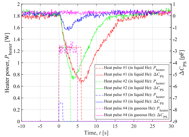
Figure 4. RC5 stray capacitance measurement in presence of local heat deposition. Measured \Delta C_{\text{PS}} and spot-heater power calculated from the measured heater current ( P_{\text{heater}} = R_{\text{heater}} I_{\text{heater}}^2 , with R_{\text{heater}} = 3.6 \Omega ), versus time. Comparison between tests conducted in liquid and in gaseous helium for various heat-pulse amplitudes and durations.
