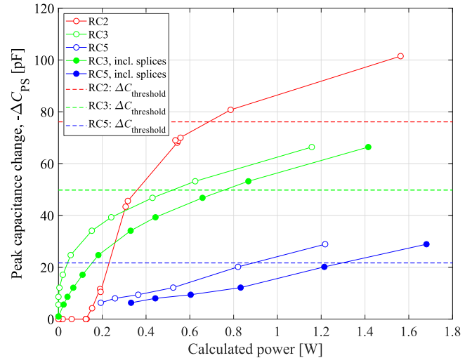
Figure 8. Measured P–S capacitance change versus power deposited in the coil, calculated from measured \Delta U I_m and (\Delta U + \Delta U_{splices}) I_m . Data obtained from three different Bi-2212 coils in liquid helium at T_{bath} = 4.2 K, during 120 s long plateaux at constant current. \Delta C thresholds selected for each coil (see table 5) are indicated with dashed lines.
