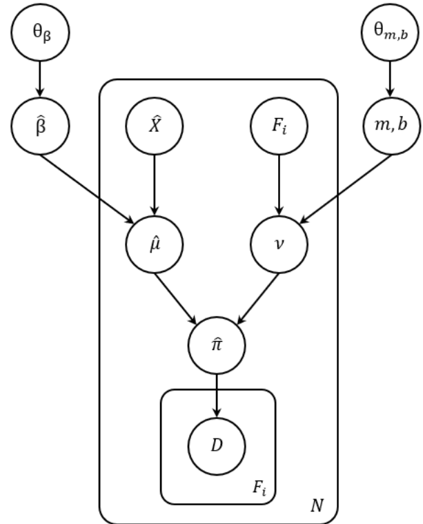
Figure 1: Graphical representation of our hierarchical Bayesian model architecture. \hat{X} , F_i , and D are all data points. \theta_\beta and \theta_{m,b} are unininformative normal priors centered at zero with a standard deviation of ten. \hat{\beta} , \hat{\mu} , \nu , m , and b are all latent model parameters.
