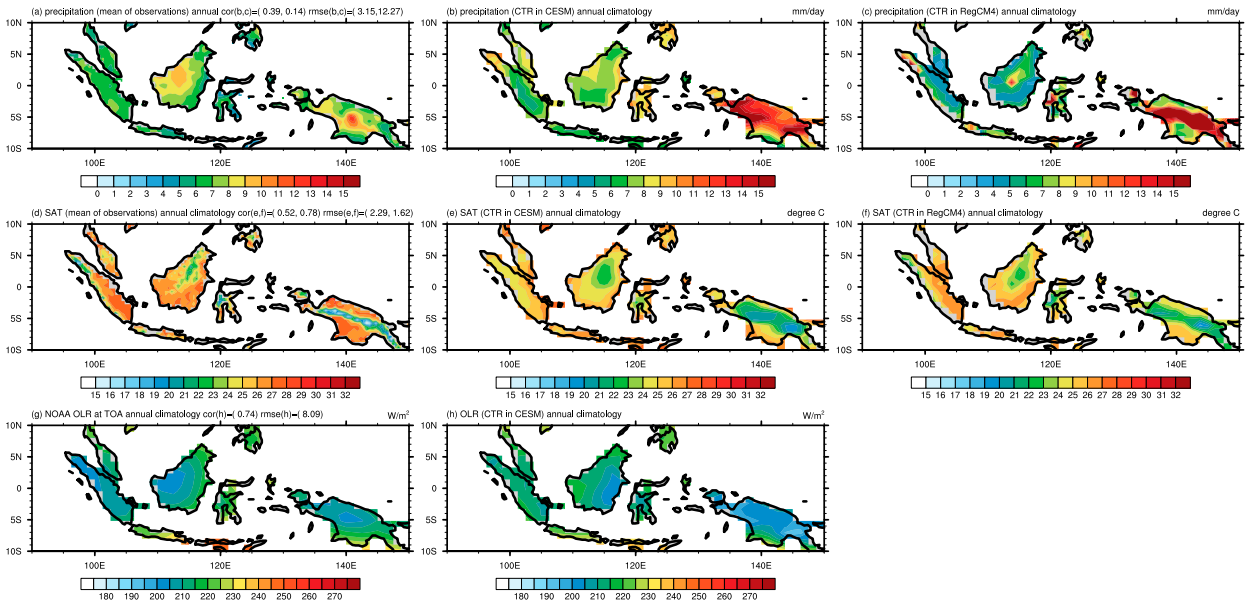
FIG. 2. Annual mean precipitation ( \text{mm day}^{-1} ) from (a) the average of four observed precipitation datasets, (b) the CESM control run (25-yr average), and (c) RegCM4 (20-yr average). Also shown are annual mean near-surface temperature ( ^{\circ}\text{C} ) from (d) the average of two observed datasets, (e) CESM control run (25-yr average), and (f) RegCM4 (20-yr average), and annual mean top of atmosphere outgoing longwave radiation ( \text{W m}^{-2} ) from (g) the observation and (h) the CESM control run (25-yr average).
