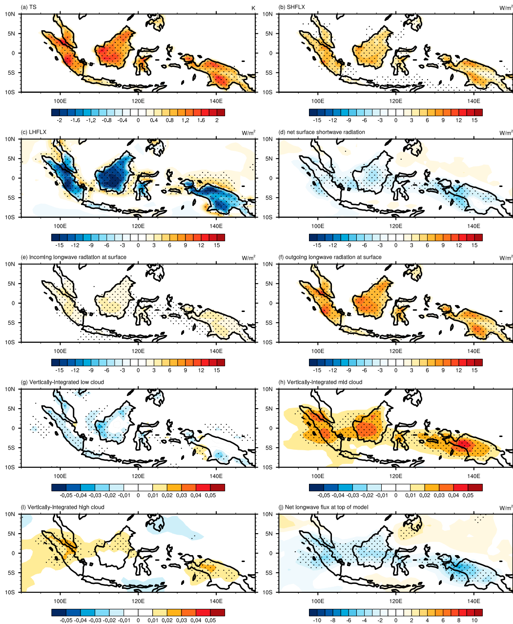
FIG. 3. Difference between deforestation experimental run and control run (DEF minus CTR) in annual mean (a) surface temperature (K), (b) surface sensible heat flux ( \text{W m}^{-2} ), (c) surface latent heat flux ( \text{W m}^{-2} ), (d) net shortwave flux at surface ( \text{W m}^{-2} ), (e) incoming longwave flux at surface ( \text{W m}^{-2} ), (f) outgoing longwave flux at surface ( \text{W m}^{-2} ), (g) vertically integrated low cloud cover, (h) vertically integrated midcloud cover, (i) vertically integrated high cloud cover, and (j) top of atmosphere outgoing longwave flux ( \text{W m}^{-2} ). Dotted areas indicate p < 0.05 .
