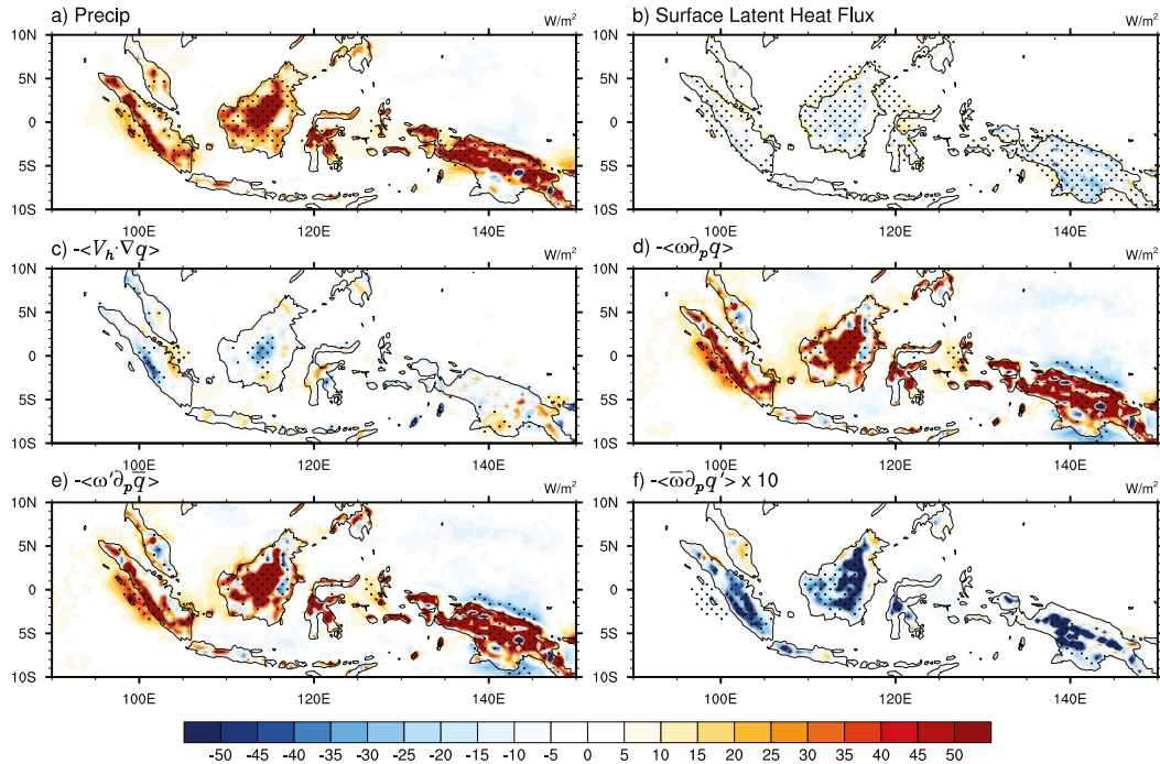
FIG. 6. As in Fig. 5, but for the results in RegCM4. Note that all the values in (f) are multiplied by 10.
