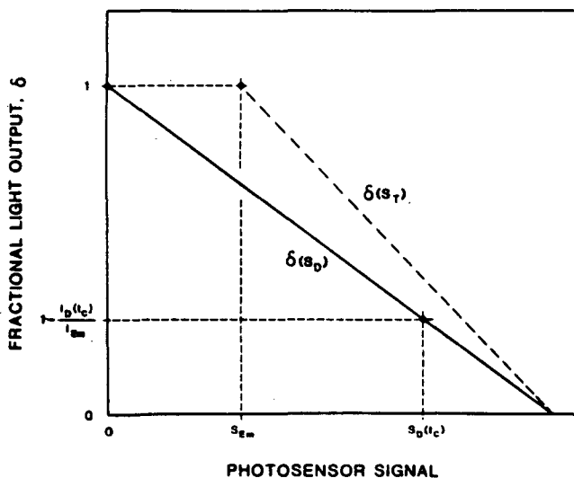
Figure 4. Relationship between fractional light output and total photosensor signal ( \delta(s_T) ) for system using sliding set-point algorithm. Solid line ( \delta(s_p) ) shows response of system to daylight component.
