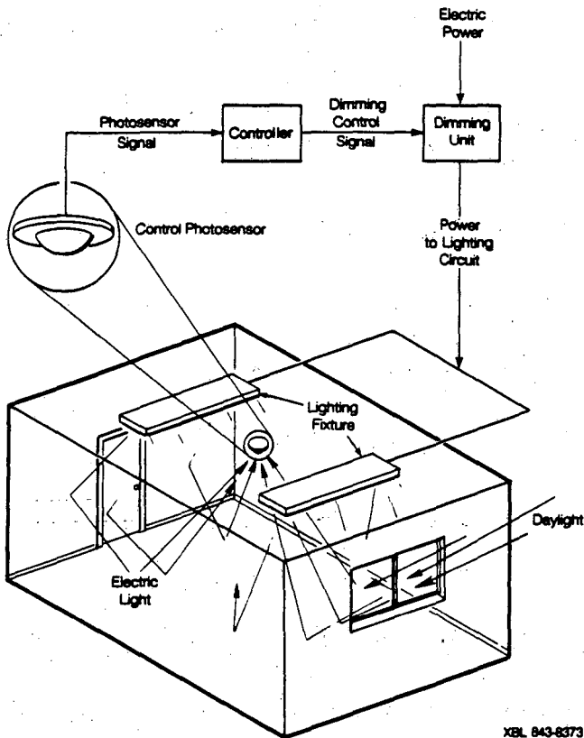
Figure 1. Schematic representation showing the relationship between the components of a photo-electric dimming system in a typical building application. The ceiling-mounted photosensor shown here is sensitive to electric light within the space as well as daylight.
