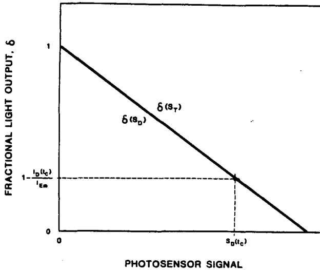
Figure 3. System response to photosensor signal for system using open-loop proportional control algorithm.
