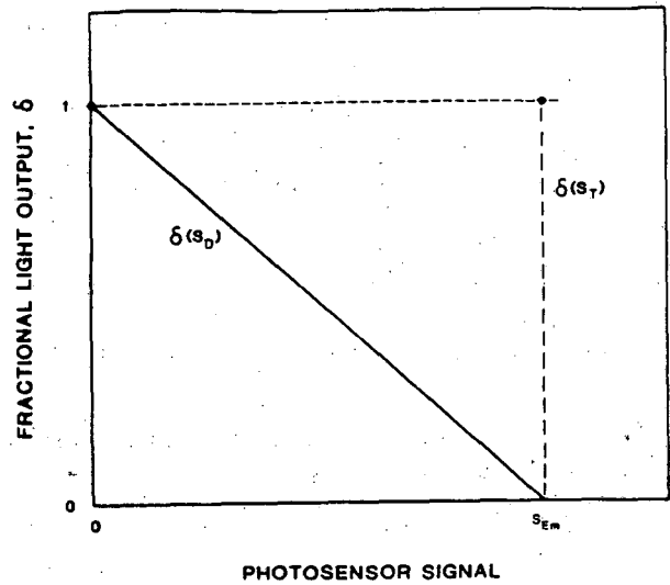
Figure 2. Relationship between fractional light output and total photosensor signal ( \delta(S_T) ) for system using constant set-point algorithm. Solid line ( \delta(S_D) ) shows response of system to daylight component.
