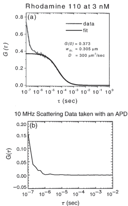
FIG. 4. Photon mode autocorrelation data taken with a 10 MHz clock frequency. (a) Rhodamine data (courtesy of Dr. Yan Chen) depicting APD afterpulsing correlation on the order of 50 ns. The correlation due to the diffusion of Rhodamine through the excitation volume is on the order of 50 \mu s. The autocorrelation decays to zero indicating no correlation for long time scales. (b) Autocorrelation of scattered laser light data which corroborates the premise that the 50 ns correlation is due to detector afterpulsing and not due to fast kinetics. Without afterpulsing the scatter data would not exhibit any correlation on the time scales measured.
