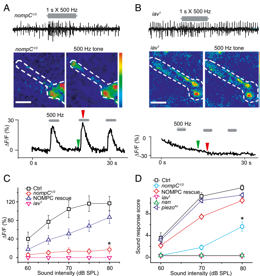
Fig. 4. TRP channel mutants affect the response of Cho neurons to sound. (A) nompC mutant exhibited reduced action potential firing and Ca^{2+} response to pure tone sound. The green arrow indicates the time of the prestimulation image; the red arrow, the 500-Hz tone. (Color range: 0–255; scale bar: 10 \mu m.) (B) Cho neurons of iav 1 showed no detectable action potential firing or Ca^{2+} response to sound. The green arrow indicates the time of the prestimulation image; the red arrow, the 500-Hz tone. (Color range: 0–255; scale bar: 10 \mu m.) (C) The Ca^{2+} response of Cho neurons in TRP channel mutants to sounds of varying intensity. WT NOMPC partially rescued the response of nompC mutant. Ctrl, NOMPC-Gal4; UAS-GCaMP5, UAS-mCherry. nompC 1/3 : nompC 1/3 ; NOMPC-Gal4, UAS-GCaMP5, UAS-mCherry. NOMPC rescue: nompC 1/3 ; NOMPC-Gal4, UAS-NOMPC/UAS-GCaMP5, UAS-mCherry. iav : iav 1 ; NOMPC-Gal4, UAS-GCaMP5, UAS-mCherry. n = 7, 7, 7, 8 (Top to Bottom). * P < 0.001, unpaired t test between Ctrl and nompC 1/3 . (D) Startle response of TRP channel and dmpiezo mutants to varying sound intensities. iav and nan mutants larval showed no response to sound. The nompC mutant demonstrated reduced sensitivity to sound, which could be rescued by the expression of WT NOMPC in Cho neurons. The dmpiezo mutant exhibited a normal response. Ctrl: w1118. nompC 1/3 : nompC 1/3 ; NOMPC-Gal4, UAS-NOMPC. iav : iav 1 . nan : nan 36 . dmpiezo : dmpiezo ko . n = 7, 7, 7, 8, 6 (Top to Bottom). * P < 0.001, unpaired t test comparing Ctrl and nompC 1/3 . Error bars represent SEM.
