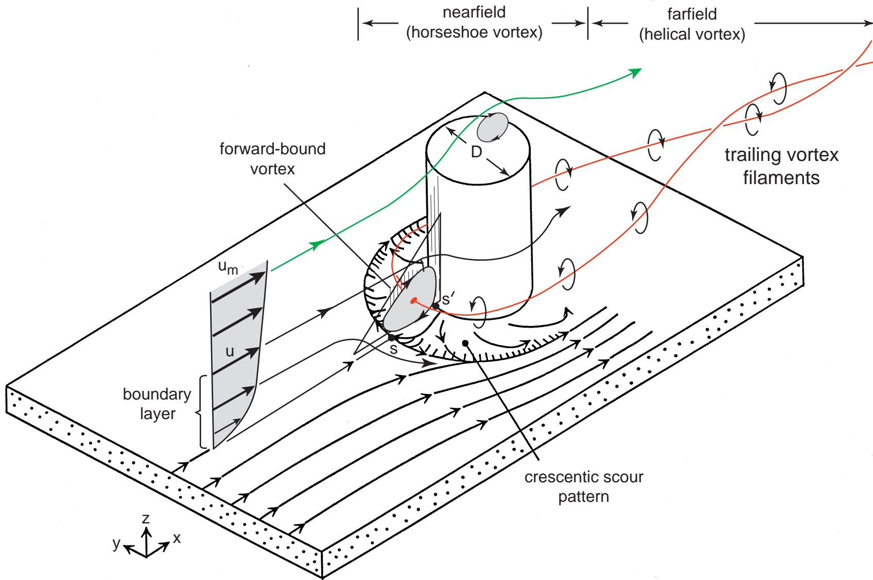
Figure 3-4. Definition sketch of fluid motion and scour features around an upright cylinder extending through the surface of a sediment bed under unidirectional flow [after Schlichting, 1979; Allen, 1984]; compare with Figure 3-1. [from Inman and Jenkins, in press 2002a]
