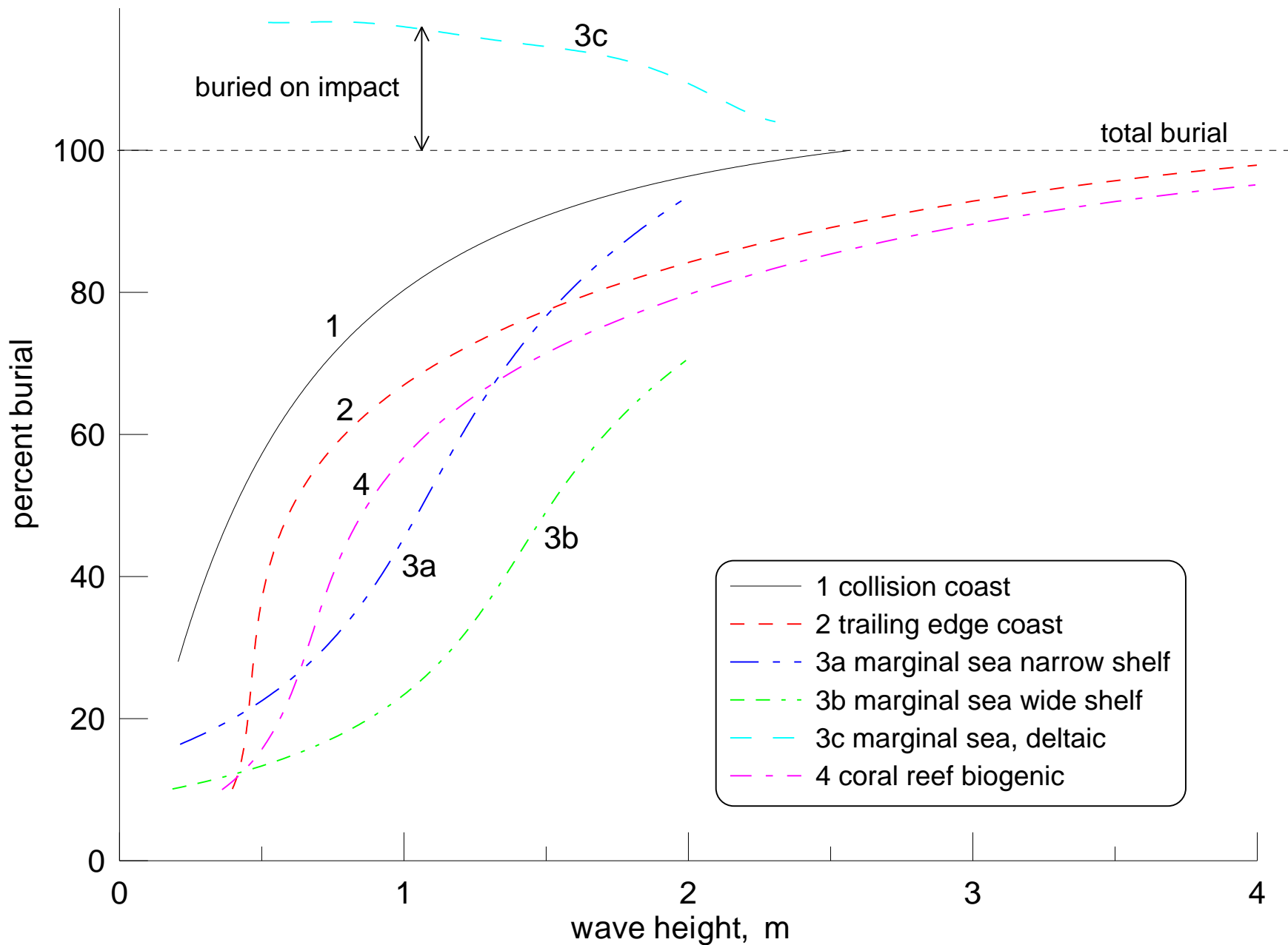
Figure 4-13. Predicted 30-day burial by waves of a MARK 52 mine in water depth of 7 m along various types of exposed coast. Closure depth, sediment type and bottom roughness from Table 4-1, wave forcing from Table A-1.
