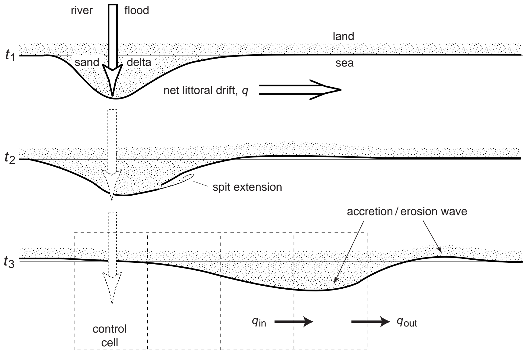
Figure 4-6. Formation of accretion/erosion wave down-drift from an episodically formed sand delta at time t_1 , where t_1 < t_2 \ll t_3 . Control cells shown by dashed lines with local balance of sediment flux q_{in} vs q_{out} . [after Inman, in press 2002]
