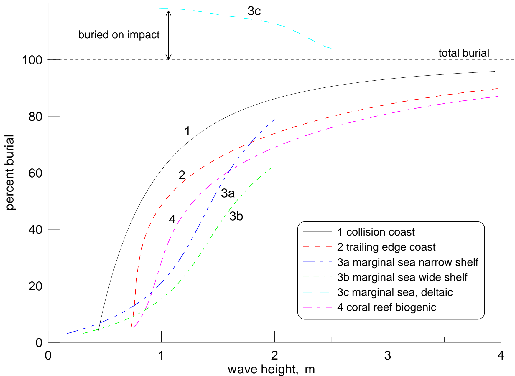
Figure 4-14. Predicted 30-day burial by waves of a MANTA mine in water depth of 7 m along various types of exposed coast. Closure depth, sediment type and bottom roughness from Table 4-1, wave forcing from Table A-1.
