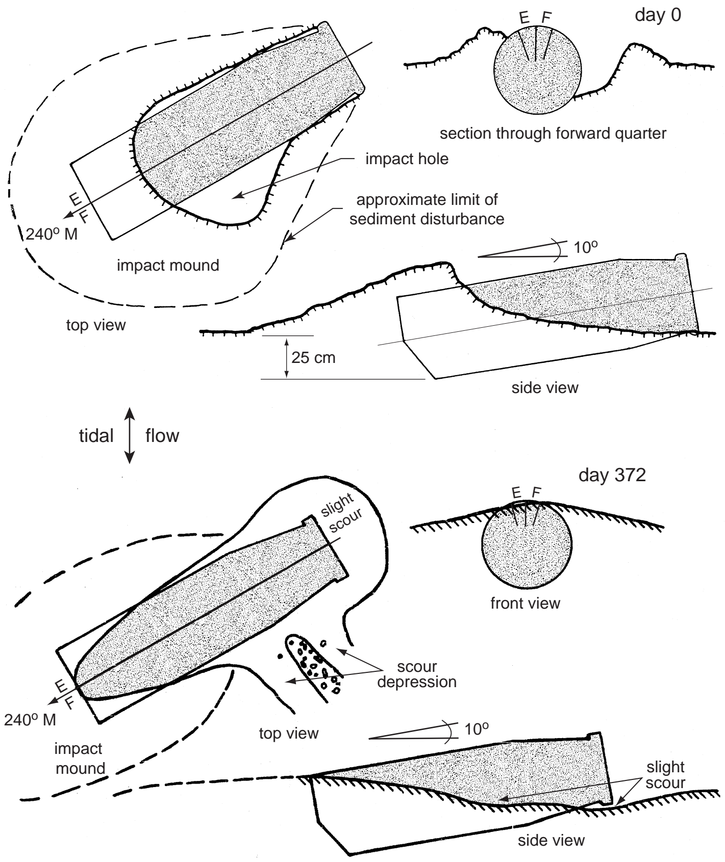
Figure 2-16. Scour pattern for HM MARK 36 mine in oscillatory tidal current, depth 8 m, bottom shell fragments over clayey silt [day 0 after Donohue and Garrison, 1954; (Able area); day 372 after McMaster et al., 1955]
