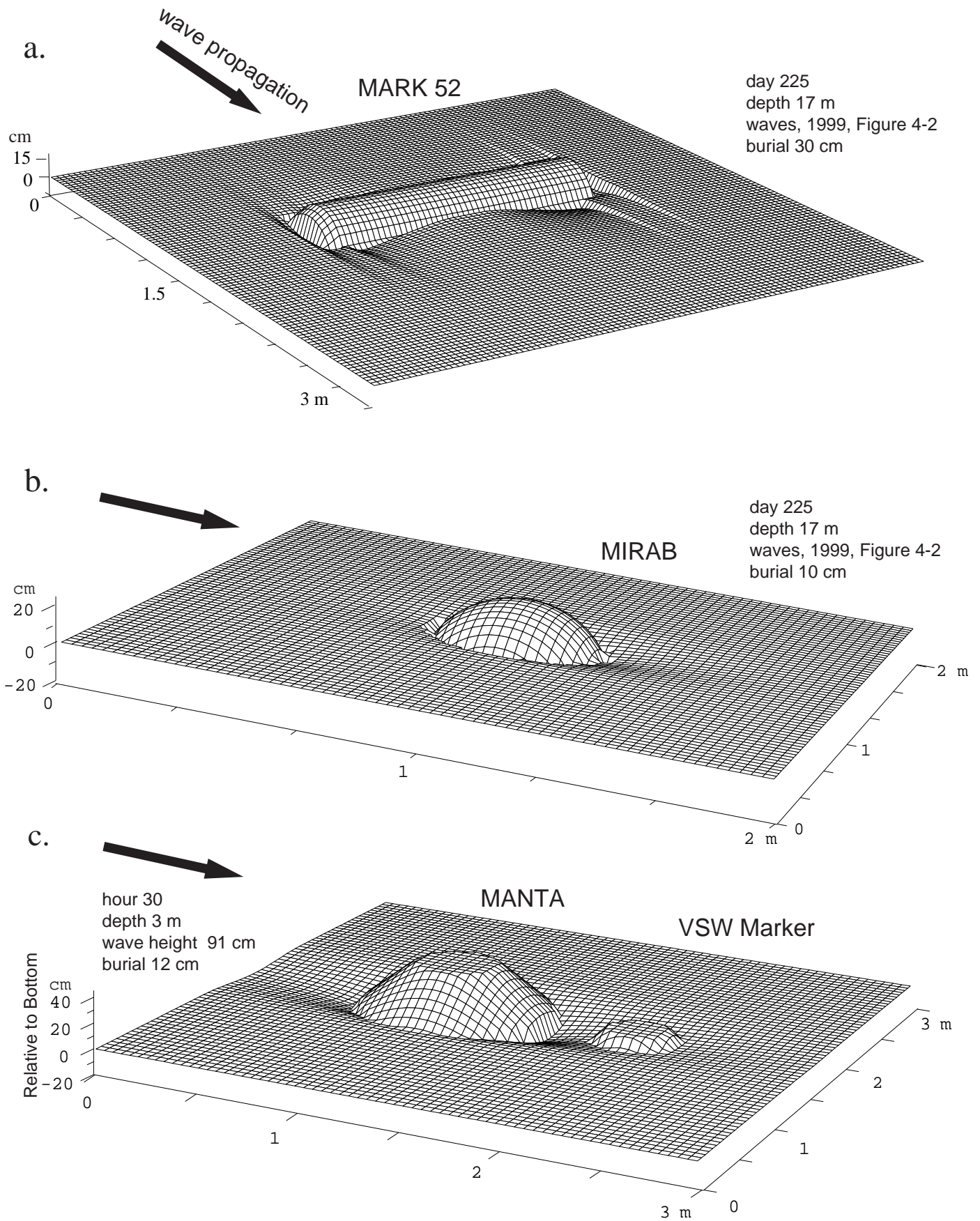
Figure 4-10. Examples of shape resolution by the VORTEX Model. Scour burial for a) cylinder, b) oblate hemispheroid, and c) truncated cones.
