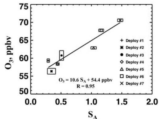
Figure 6. Correlation between \text{O}_3 and IR aerosol scattering ratios during TOPSE in mid troposphere (4–6 km) and at high latitudes (60°–85°N). Size of rectangles represents the standard error in the mean value of \text{O}_3 and aerosol scattering ratios for each deployment.
