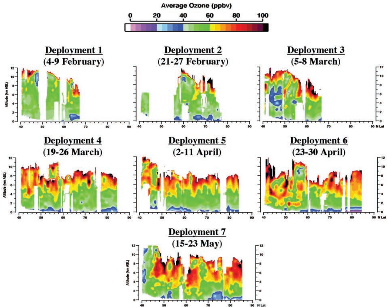
Figure 2. Average O_3 distributions observed on each deployment during TOPSE.
