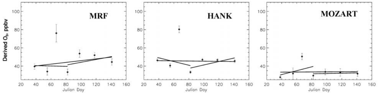
Figure 10. Ozone trend in 60°–85°N, 4–6 km region calculated from PV \times O_3/PV , where PV is derived from MRF, HANK, and MOZART models, and O_3/PV is from the time-dependent average O_3/PV ratio in lower stratosphere ( PV = 7 PVU) (Klonecki et al., submitted manuscript, 2002) (upper plots) and from the O_3/PV ratio from Resolute (280 mb, PV = 5 –6 PVU) (lower plots).
