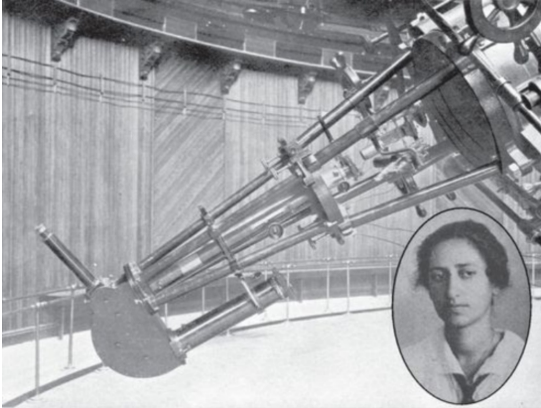
A photograph, reproduced from Campbell, of the original Mills spectrograph on the 36-inch refractor at Lick Observatory as used by Mary Lea Heger for her observations of the first DIBs. (Photo: 1919 Blue & Gold Yearbook, Bancroft Library, UC Berkeley)
