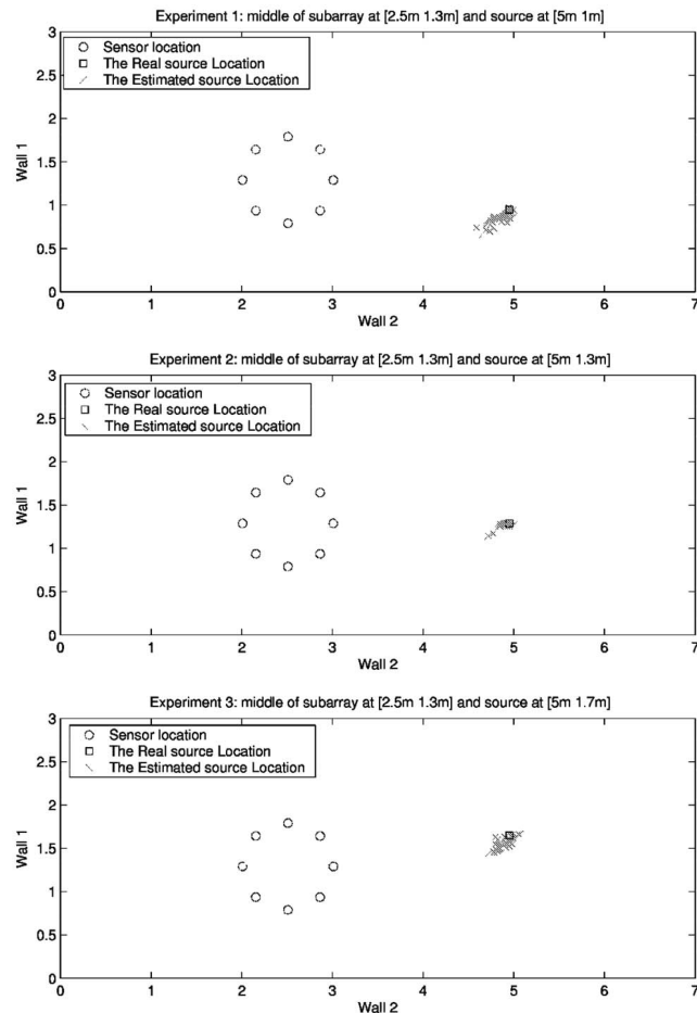
Fig. 22. Circular subarray: Experiments 1, 2, and 3.
