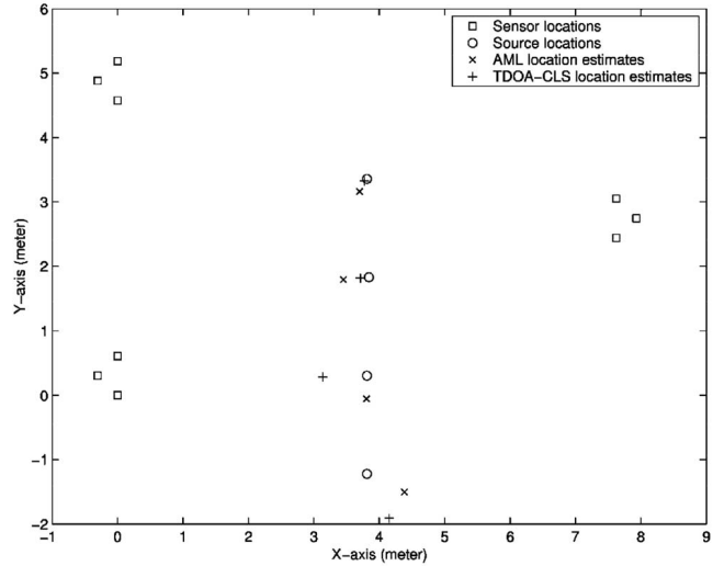
Fig. 10. Bearing crossing localization results of a vehicle source at different locations.
