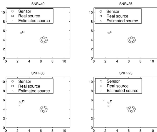
Fig. 20. Simulation results for different SNR when the centroid of the subarray is at [6.5\text{m } 4\text{m}] and the source is at (4\pi/6\text{rad}, 2\sqrt{3}\text{m}) relative to the subarray.
