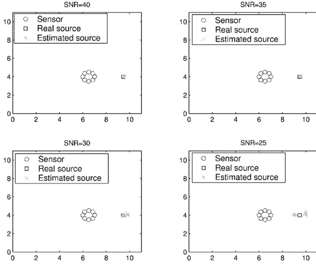
Fig. 19. Simulation results for different SNR when the centroid of the subarray is at [6.5\text{m } 4\text{m}] and the source is at (0\text{rad}, 2\sqrt{3}\text{m}) relative to the subarray.
