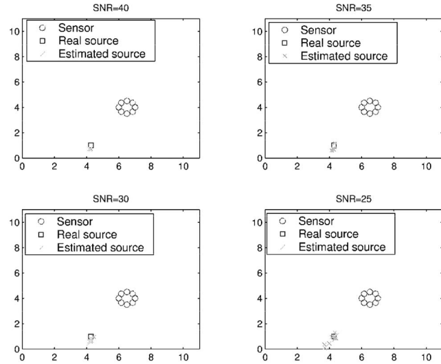
Fig. 21. Simulation results for different SNR when the centroid of the subarray is at [6.5\text{m } 4\text{m}] and the source is at (4\pi/3\text{rad}, 2\sqrt{3}\text{m}) relative to the subarray.
