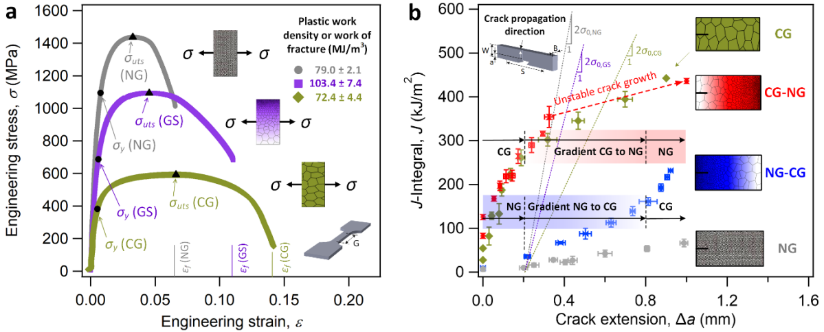
FIGURE 2 Mechanical properties of the uniform grain-sized pure NG and pure CG structures, and gradient structured (CG \rightarrow NG and NG \rightarrow CG) Ni at room temperature. (a) Uniaxial tensile properties of NG specimen show an increase in both yield strength and ultimate tensile strength compared to those in CG specimen. A good combination of strength and ductility can be achieved in the GS specimen as confirmed by the increase of plastic work density (or work of fracture), i.e. , the area under the true stress-plastic strain curve, in the GS specimen from those in the CG and NG specimens. (b) R -curves for the four structures presented in terms of J -integral as a function of crack extension \Delta a . As the crack grows to \Delta a = 1 mm, the J -integral value of the CG specimen is increased to 442 kJ.m^{-2} , some six times higher than that of the NG sample, 63 kJ.m^{-2} , showing evidence of ductile and brittle crack-growth behavior in the CG and NG structures, respectively. The R -curve of the gradient NG \rightarrow CG materials shows an increasing slope, compared to that of the pure NG structure, as the crack grows into the gradient region, indicating an enhanced crack-growth toughness. The gradient CG \rightarrow NG specimen presents a similar crack resistance to the CG specimen until crack extension ends in the initial part of the gradient zone, whereupon unstable crack growth occurs into the nano-grained region. A transition in the fracture mode from ductile to “brittle” is apparent as the crack proceeds through the CG \rightarrow NG gradient in this material.
