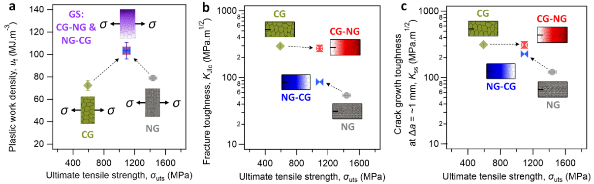
FIGURE 8 Strength vs. toughness. (a) Plot showing the plastic work density during uniaxial tensile fracture as a function of the ultimate strength, (b) Ashby map showing the fracture toughness K_{JIC} at crack initiation as a function of the ultimate tensile strength for the CG, NG, CG→NG, and NG→CG Ni structures, and (c) Ashby map showing the crack growth fracture toughness K_{SS} at \Delta a \sim 1 mm as a function of the ultimate tensile strength for the CG, NG, CG→NG, and NG→CG Ni structures.
