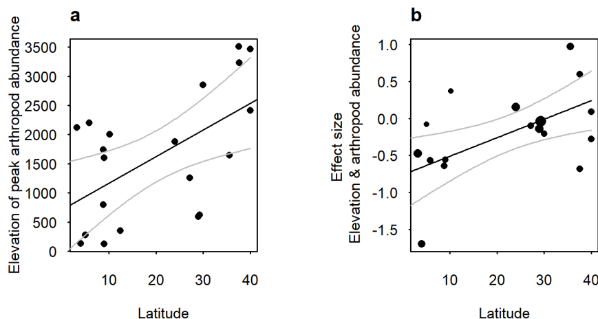
Figure 3. a Relationship between elevation of peak arthropod abundance and latitude; b Relationship between effect size of the correlation between arthropod abundance and elevation and latitude. Size of each point indicates sample size of the gradient. Grey lines in both plots indicate 95% confidence interval.
