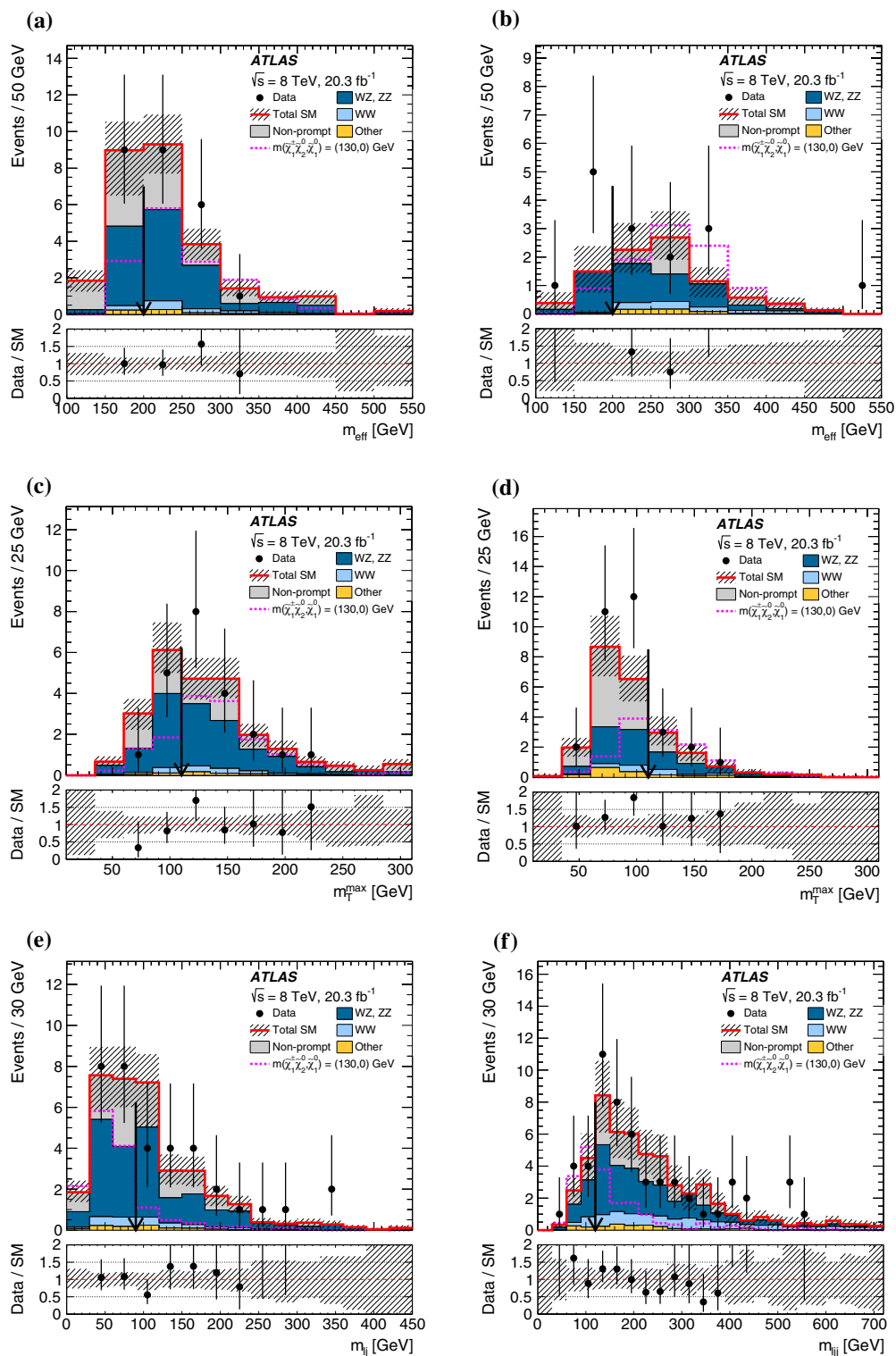
Fig. 6 Distributions of effective mass m_{\text{eff}} , largest transverse mass m_{\text{T}}^{\text{max}} , invariant mass of lepton and jets m_{\ell j} and m_{\ell j j} for the same-sign dilepton channel with one jet (left) and two or three jets (right). SRll-1 is the sum of SRll-1, SRll-1, and SRll-1; SRll-2 is the sum of SRll-2, SRll-2, and SRll-2. All selection criteria are applied, except for the one on the variable being shown. The vertical arrows indicate the boundaries of the signal regions, which may not apply to all flavour channels. The hashed areas represent the
