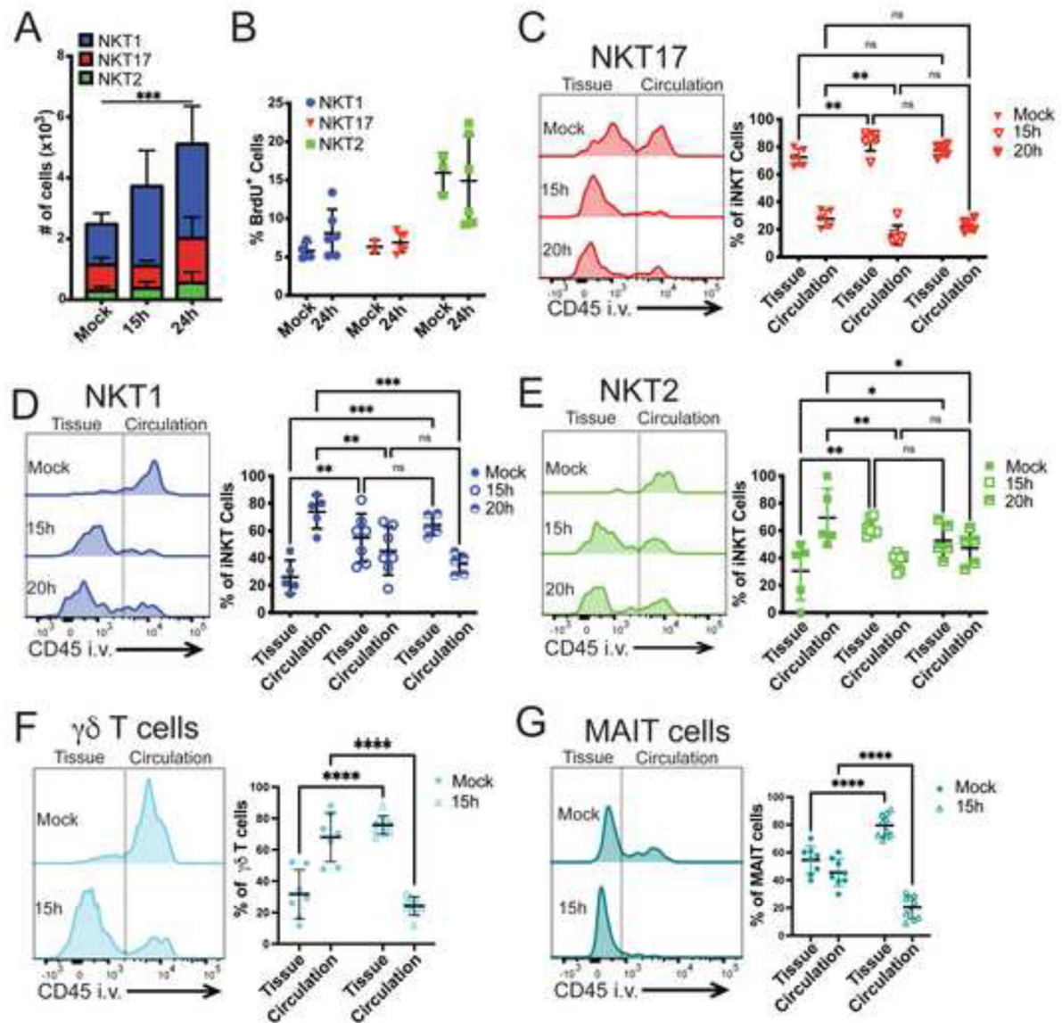
Figure 1: Innate-like T cells are recruited into the lung tissue after S. pneumoniae infection.
