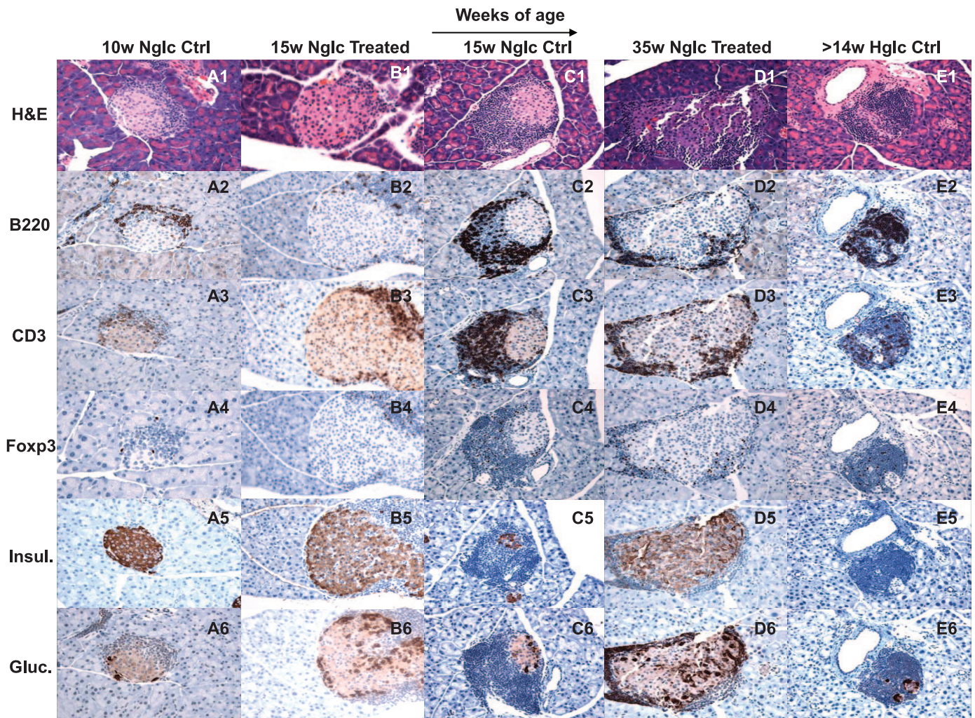
FIG. 3. Histology of prevention studies. At baseline, NOD mice showed mild perinsulitis (A1) with many B220 + cells (A2) and some CD3 + cells (A3) but still with well-preserved insulin and glucagon staining (A5 and A6). FoxP3 + cells are merely present at baseline (A4). Interestingly, at 15 weeks of age, treated NOD mice showed reduced infiltrate (B1) with no B220 + cells (B2) and fewer CD3 + cells (B3), whereas in the control, B220 + and CD3 + cells are abundantly represented with increased infiltrate (C1–C3). At 35 weeks of age, the treated group showed cleaner pancreata compared with the untreated control hyperglycemic NOD mice (D1 and E1). B220 + and CD3 + cells did not infiltrate the islets in the treated group (D2 and D3), whereas in the controls, islets were extensively infiltrated by B220 + and CD3 + cells (E2 and E3). Islet morphology is well-preserved in the treated group at 15 and 35 weeks of age (B5, B6, D5, and D6) but not in the control group (C5, C6, E5, and E6). FoxP3 staining of islet infiltrate revealed a persistent reduced expression of FoxP3 in untreated compared with treated NOD mice at 15 and 35 weeks of age, particularly when compared with the massive presence of T-cells in the control (B4, D4, C4, and E4). (Please see http://dx.doi.org/10.2337/db08-0420 for a high-quality digital representation of this image.)
