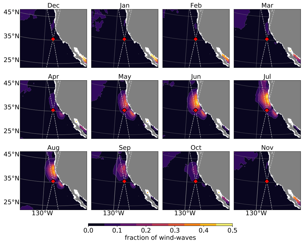
Figure 9. Monthly average of the fraction of days with c_p/U_{10} \leq 1.2 , which is associated wind-sea dominated sea states. The monthly maps were computed using peak phase speed and wind speed from the WW3 hindcast.
