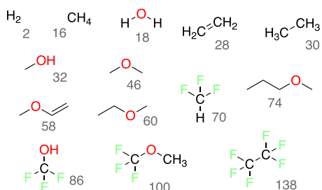
Figure 2. Gases predicted to evolve from \text{Mg}(\text{TFSI})_2/\text{G2} electrolytes based on CRN analysis and prediction of solubility S_{\text{G2}} . The mass of each CRN product (rounded, in amu) is shown next to the 2D structure in gray.
