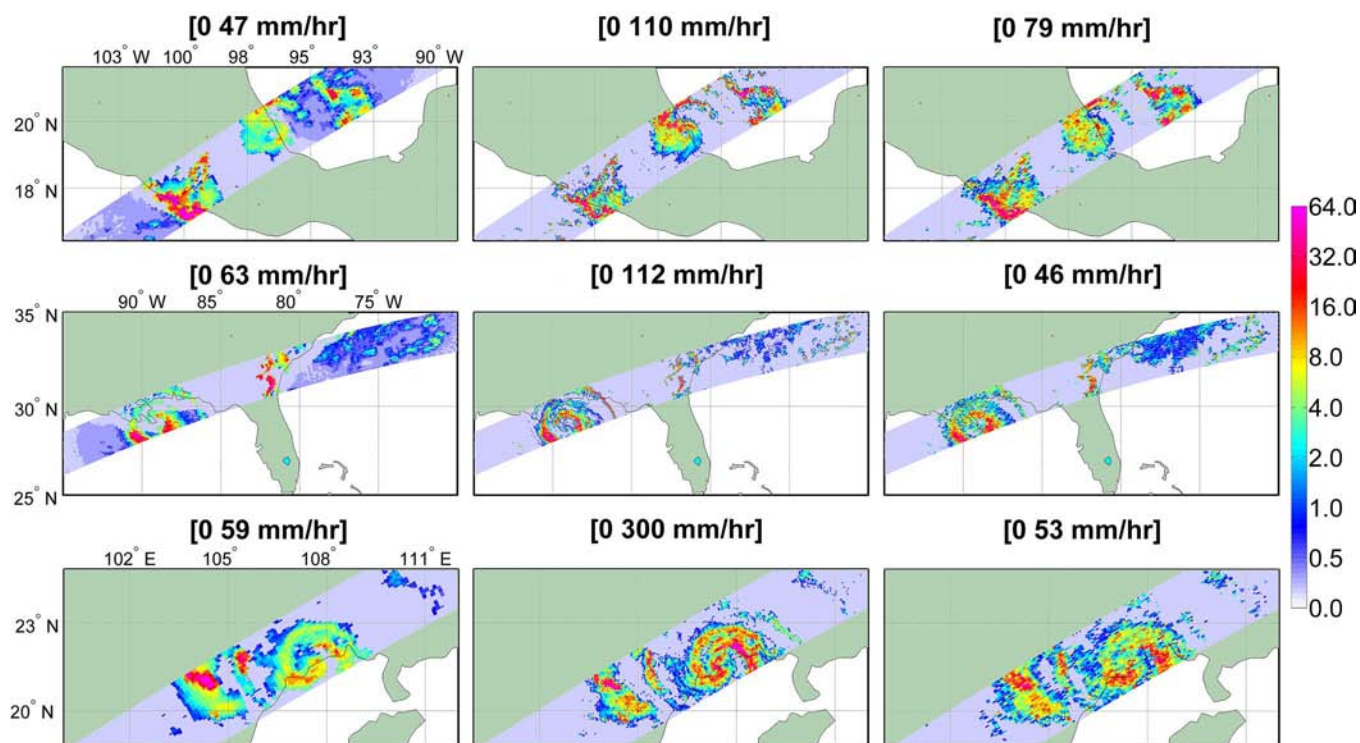
Fig. 8. (Left to right) TMI-2A12, PR-2A25, and ShARP retrievals. (Top to bottom panels) Tropical storm Fernand in 08/26/2013 (orbit no. 89874) at 05:30 UTC, hurricane Isaac on 08/28/2012 (orbit no. 84227) at 22:12 UTC, and typhoon Kai-tak in 08/17/2012 (orbit no. 84050) at 13:35 UTC.
