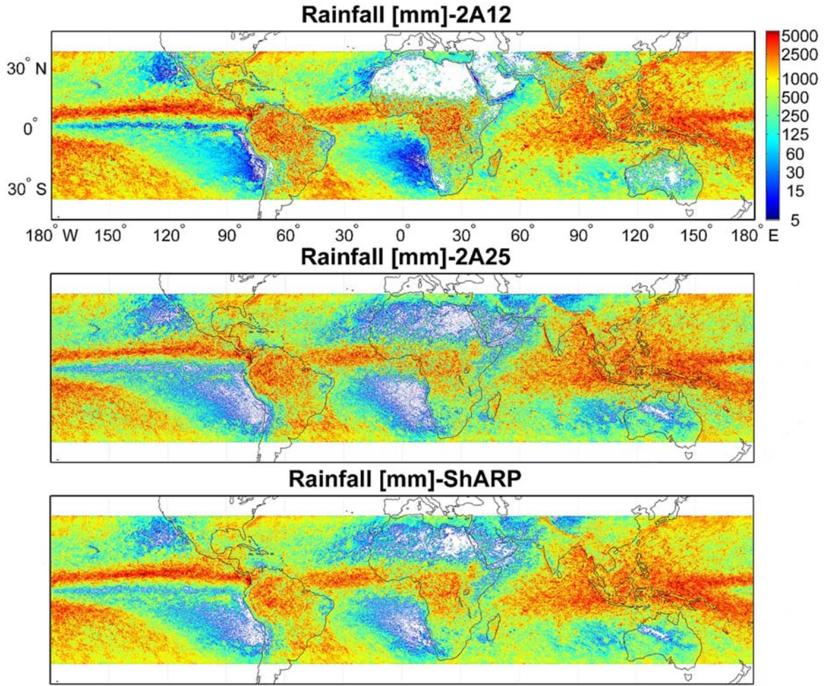
Fig. 11. Annual estimates of the total rainfall (in millimeters) in 2013 mapped onto a 0.1^\circ grid box. (Top to bottom panels) 2A12, 2A25, and ShARP retrieval products.
