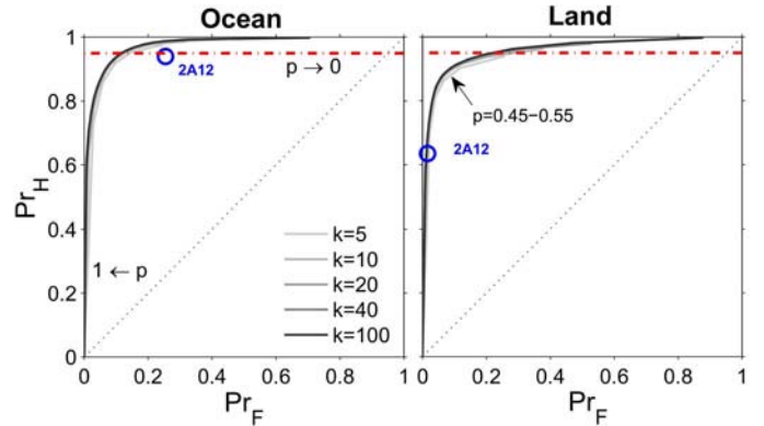
Fig. 5. Rainfall ROC curve over (left panel) ocean and (right panel) land for different probabilities of detection p \in [0, 1] and numbers of nearest neighbors K \in \{5, 10, 20, 40, 100\} of ShARP. The blue circles show the 2A12 (version 7) product, and the red dash-dotted lines show the 0.95 probability of hit as a datum.
