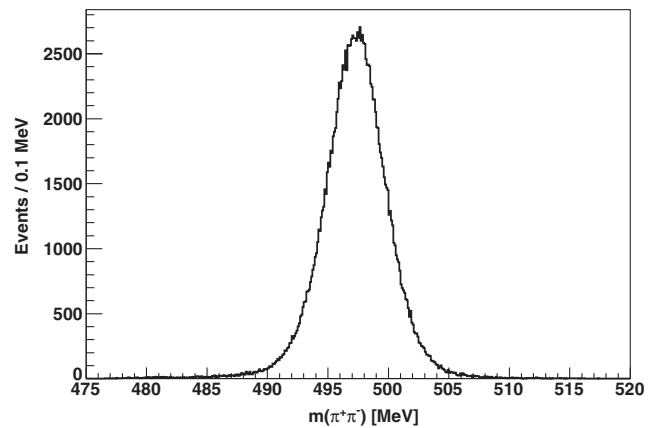
FIG. 5. Sample of K_S^0 \rightarrow \pi^+\pi^- candidates from D^{*+} \rightarrow D^0\pi^+ \rightarrow (K_S^0\pi^-\pi^+)\pi^+ decay where the K_S^0 daughter pions satisfy the same tracking criteria as the slow pions of the D^{*+} analysis.
