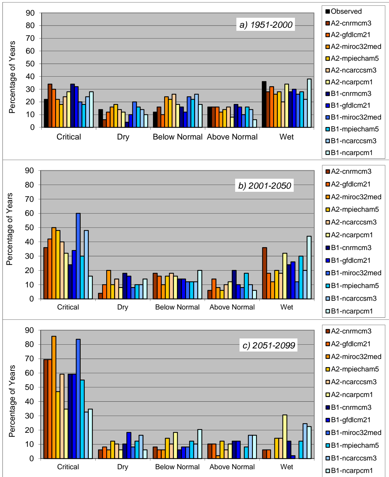
Figure 7. SJJ Relative Frequency Histograms for (a) 1951–2000, (b) 2001–2050, and (c) 2051–2099
