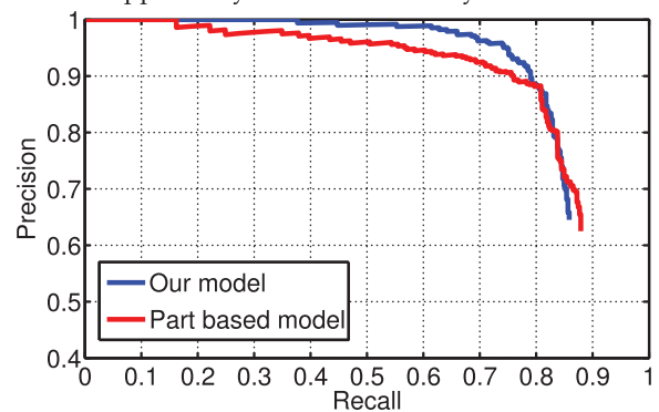
Fig. 11. We plot upper body detection on the Buffy dataset, comparing our articulated pose detector with the state-of-the-art deformable part model of [4] trained on the same data as our model.
