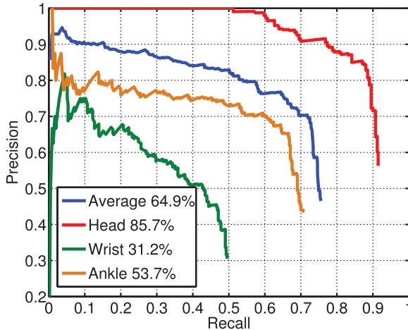
Fig. 9. We present our new evaluations of PCK and APK on the Parse test set, using a full-body model of K = 26 parts and T = 6 mixtures. PCK is the fraction of times a predicted keypoint was close to a ground-truth keypoint given a human bounding box on a test image. APK evaluates the average precision of keypoint detections obtained without access to any annotations on the test image; this requires a pose estimation algorithm to perform NMS.
