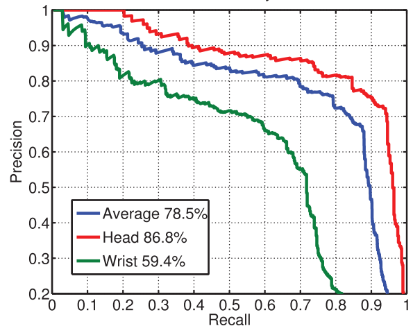
Fig. 10. We present our new evaluations of PCK and APK on the Buffy test set, using a model of K = 18 parts and T = 6 mixtures. Note that the overall average APK (across all keypoints) is 78.5 percent, indicating this test set is easier than the Parse image benchmark.
