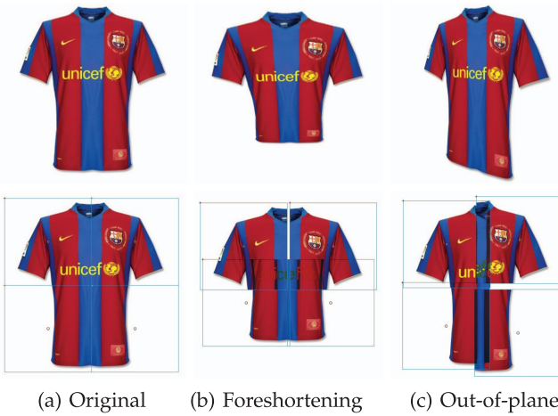
Fig. 2. We show that four small, translating parts can approximate nonaffine (e.g., perspective) warps.
