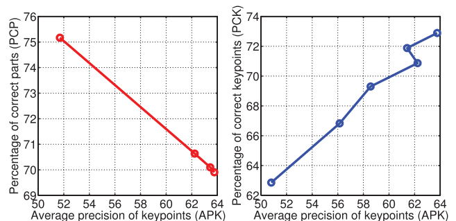
Fig. 5. We compare our “gold standard” evaluation criteria of APK with PCP and PCK. Recall that APK treats pose estimation as a body-part detection problem, and computes average precision from a precision-recall detector curve. On the left , we plot different PCP and APK values obtained by tweaking NMS strategies. By generating more candidates, one produces a low APK but an artificially high PCP (as defined in the Buffy toolkit [8]), suggesting PCP does not correlate well with our gold standard. On the right , we show that PCK correlates positively with APK.
