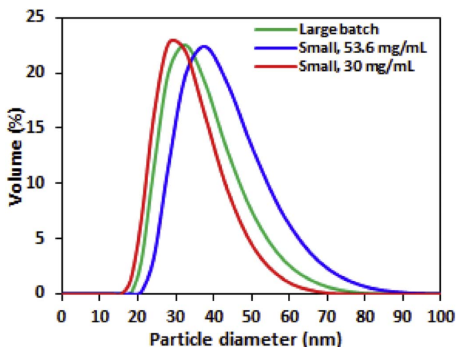
Fig. 4. Volumetric size distribution for the ANSP inks, small 30 mg mL -1 is the solid red line, small 53.6 mg mL -1 is the blue line and the large batch is the green line. (For interpretation of the references to colour in this figure legend, the reader is referred to the web version of this article.)
