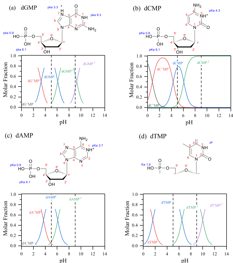
Figure 2. Fully protonated nucleotide structures and their pK_a values (top) and speciation plots determined from the Henderson–Hasselbalch equation (bottom) are shown for (a) deoxyguanosine monophosphate, dGMP; (b) deoxycytidine monophosphate, dCMP; (c) deoxyadenosine monophosphate, dAMP; and (d) deoxythymidine monophosphate, dTMP.
