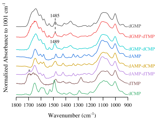
Figure 7. ATR-FTIR spectra at pH 5 of nucleotide adsorption at 180 min on TiO 2 . Single-component adsorption is shown for dGMP (black), dAMP (blue), dTMP (brown), and dCMP (green). Equimolar noncomplementary coadsorption shown for dGMP-dTMP (red) and dAMP-dCMP (gold). Equimolar complementary coadsorption shown for dGMP-dCMP (light blue) and dAMP-dTMP (purple). Spectra have been normalized to 1001 cm -1 . *Refers to the coadsorbed 1694 cm -1 \nu (C=O) due to dTMP in second layer.
