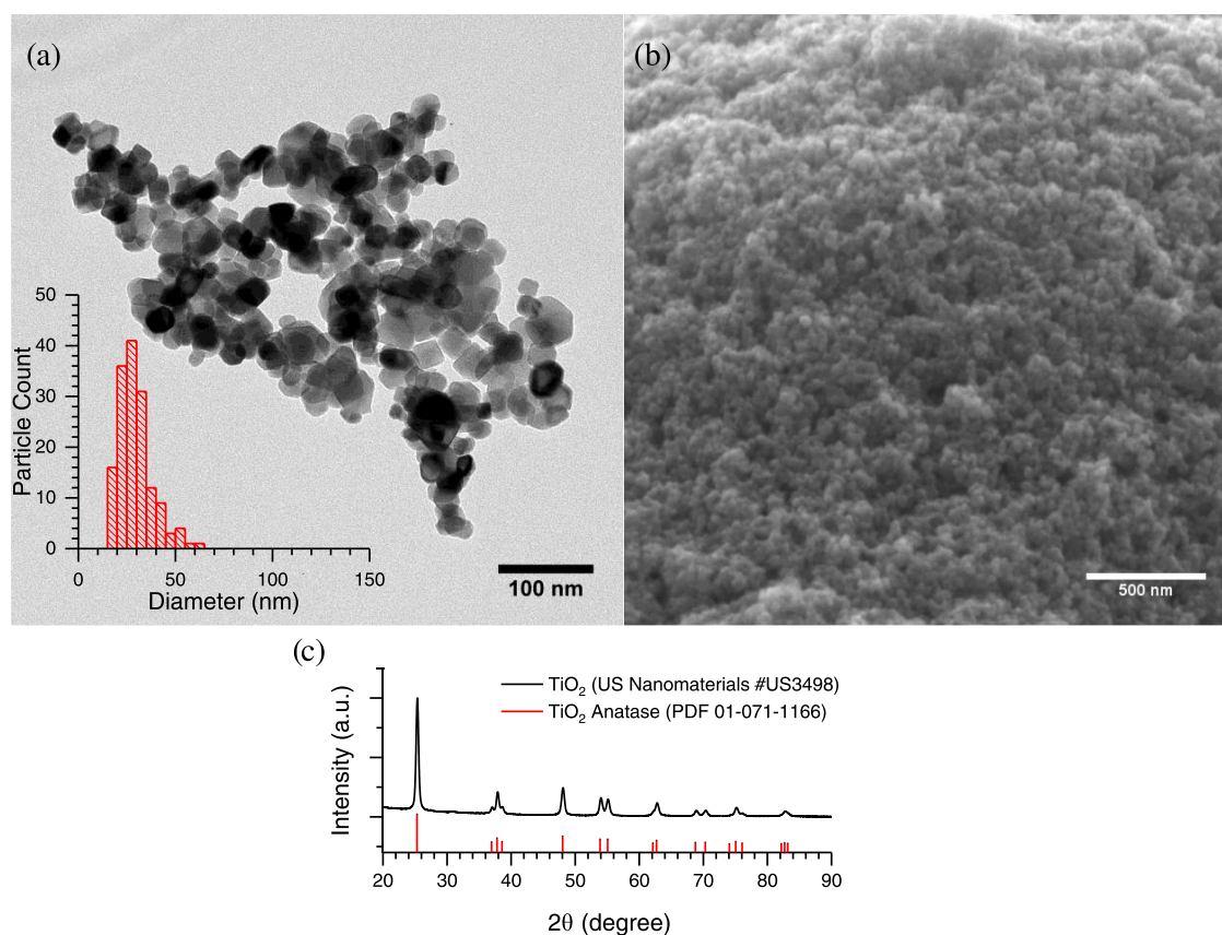
Figure 1. Particle characterization for TiO 2 particles. (a) TEM micrograph with size distribution analysis (inset); (b) SEM micrograph of a particle thin film; and (c) XRD data of anatase TiO 2 .
