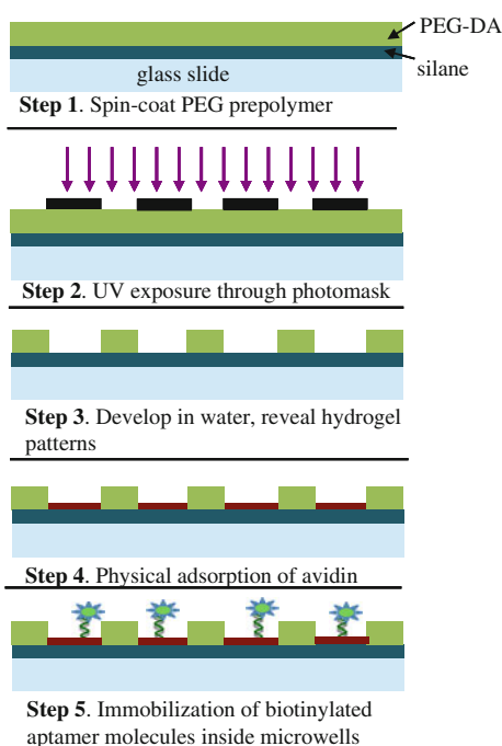
FIGURE 2. Process flow diagram for micropatterning hydrogel microwells and for immobilizing beacon molecules inside the microwells.
