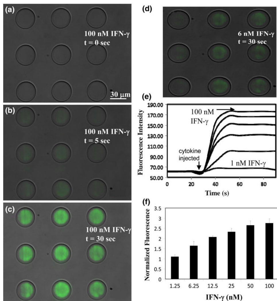
FIGURE 5. (a–c) A sequence of fluorescence/brightfield overlay images taken at different time points from a set of microwells challenged with 100 nM IFN- \gamma . Appearance of fluorescence in the microwells is due to displacement of quenching strands in the immobilized beacons by quenching strands. (d) Fluorescence response of a different set of microwells challenged with 6 nM IFN- \gamma . The signal was considerably lower than in the case of microwells challenged with 100 nM IFN- \gamma (c), proving that microwell response depended on the concentration of analyte. (e) Temporal evolution of fluorescence signal in microwells challenged with varying concentrations of IFN- \gamma . (f) A plot of signal intensity vs. IFN- \gamma concentration showing that detection limit for these sensing surfaces was 5 nM and linear range extended to 100 nM. Error bars represent standard deviation of the mean for three ( n = 3 ) separate experiments. The values for fluorescence intensity were chosen from curves in part (e) after signal saturation (e.g. t = 60 s). Fluorescence signal was normalized by background fluorescence ( F_0 ).
