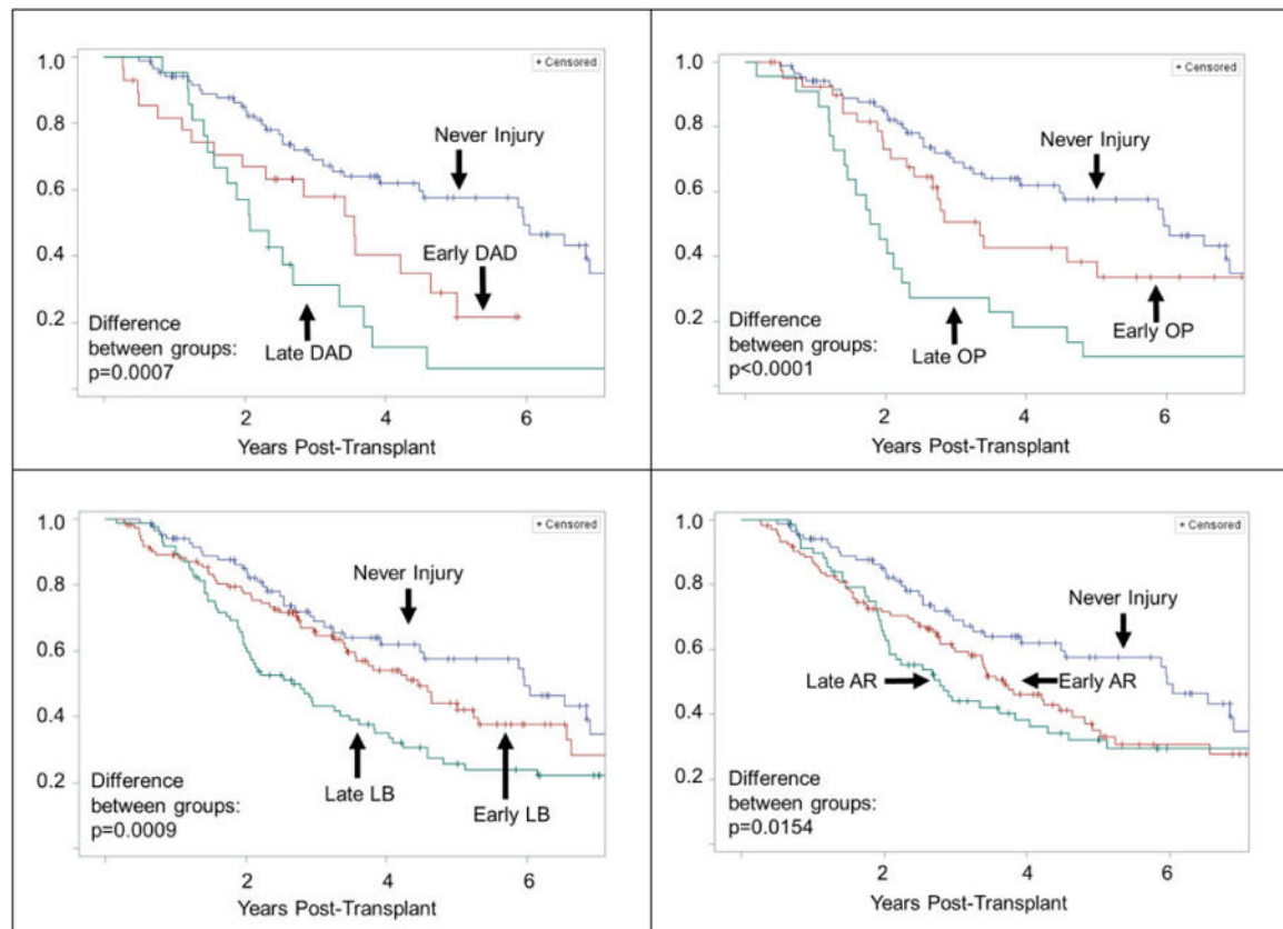
Figure 3. Kaplan-Meier plot for time to CLAD in lung transplant recipients with never vs early vs late-onset episodes of allograft injury. Early: < 6 months from transplant, late: ≥ 6 months post-transplant.
