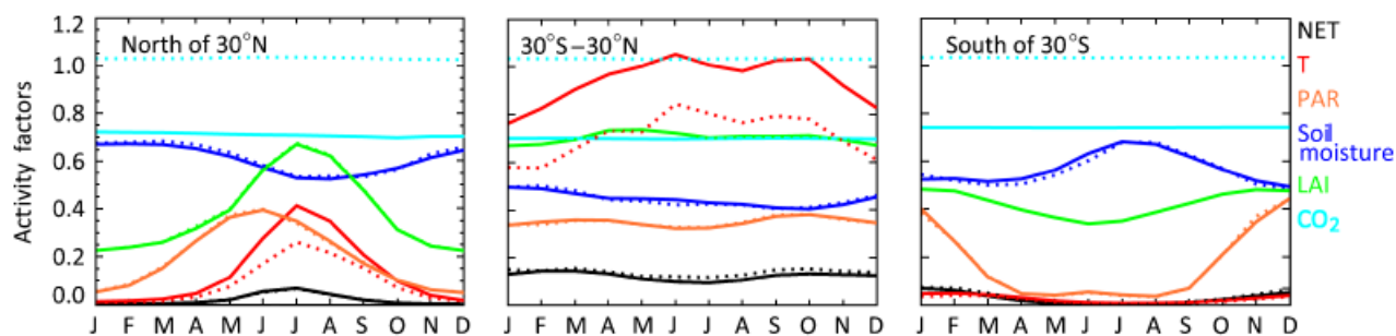
Fig. 4 Present day (2000, dotted lines) and future with fixed vegetation (2100, solid lines) seasonal cycle of mean isoprene emission activity factors North of 30°N (left), in the tropics (center) and South of 30°S (right).
