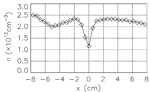
FIG. 2. Profile of the density depression at time t=32 \mu\text{s} after the bias pulse is applied to the plate electrode. The profile is obtained from ion saturation current measurements at each location along the line y=0 , and averaged over 30 plasma discharges. The measurement uncertainty is \pm 10\% and assumes a constant background electron temperature of 5.5 eV. The unbiased electrode produces a much shallower depression (within 10% of the background) at x=0 .
