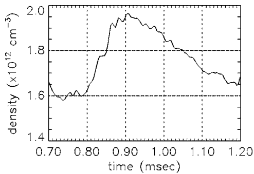
FIG. 6. Density as a function of time measured with a Langmuir probe biased to collect ion-saturation current at (x, y, z) = (0, 0, -448) cm. The time series is plotted starting at 0.7 ms after the turn on of bias voltage to the plate located at the origin. The density is averaged over an ensemble of 128 plasma discharges. The measurement assumes a constant electron temperature of 5.5 eV.
